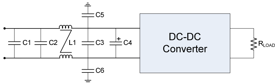
Figure 20. EMI Filter
