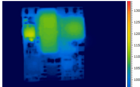
Figure 8. Thermal Image of CPZ5A48 (5A output, 70C Ambient, 200lfm airflow, Vin = 48V, T max = 115°C)
