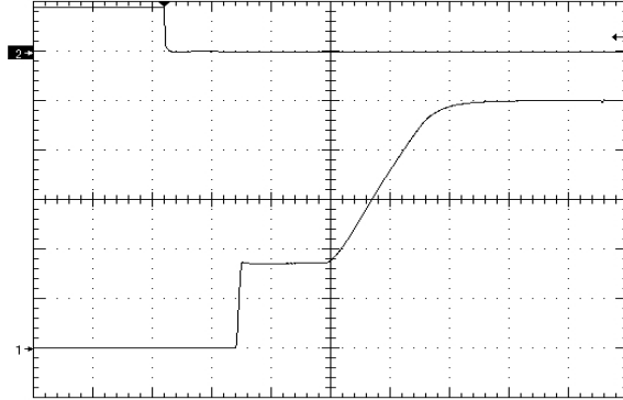
Figure 14. Startup Waveform via Enable Pin, time scale 4mS/div. Vin=Vin_nom lout=no load Cout=0, Ch1=Vout (1V/div), Ch2=enable (5V/div)
