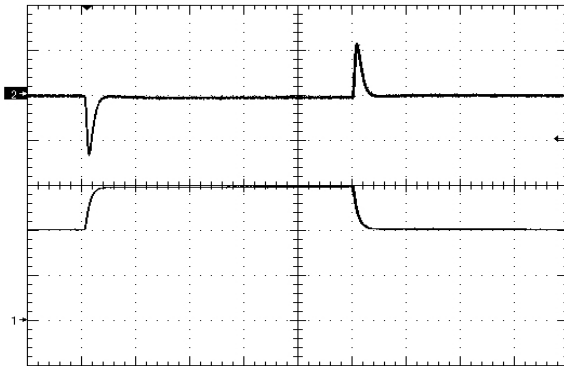
Figure 15. Load Transient Response (50mV/div), di/dt=0.1A/uS, 50% - 75% - 50% of full load, Cout=Fig3 time scale: 200uS/div. Ch1=Vout, Ch2=lout (1A/div)
