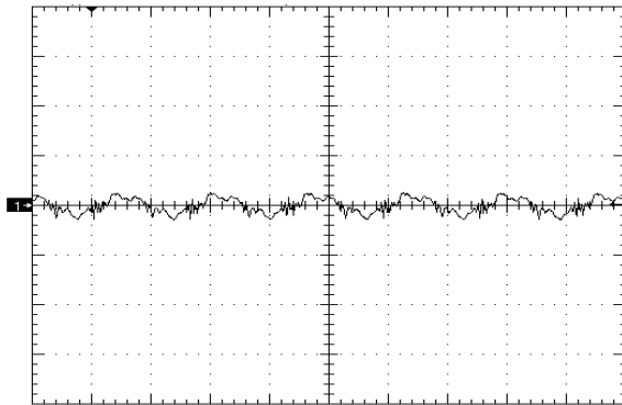
Figure 7. Output Voltage Ripple (50mV/div), time scale – 1uS/div. Vin=Vin_nom, full load Cout=1uF ceramic + 22uF Ceramic (see Fig 18)
