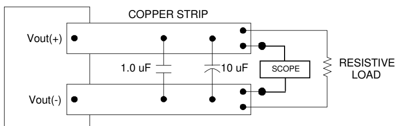
Figure 18. Peak-to-Peak Output Noise Measurement Test Setup.
