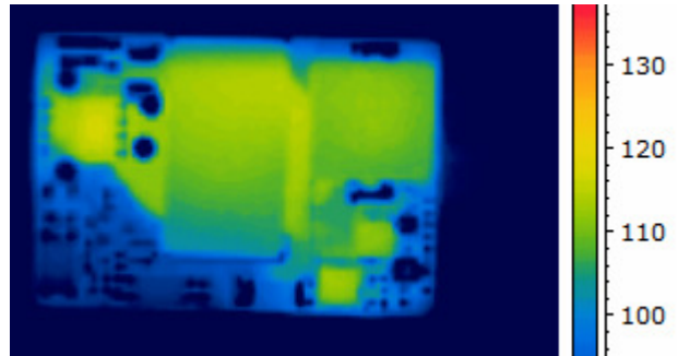
Figure 4. Thermal Image of CPT8B48 8.3A output, 55C Ambient, 200lfm airflow, Vin = 48V, airflow from pin 3 to pin 1, T max = 116°C
