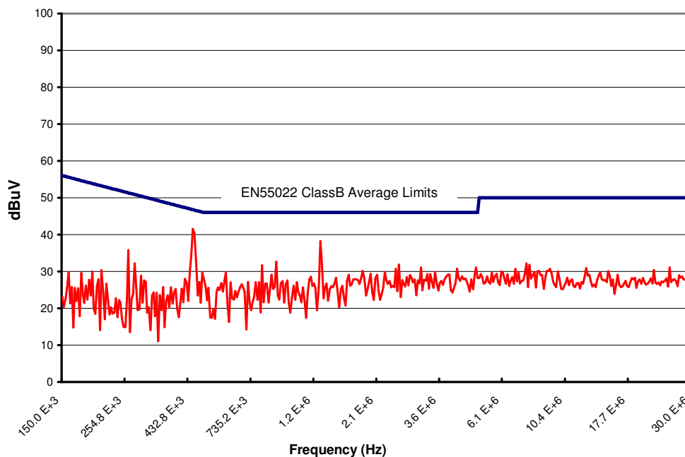
Figure 18. CPT8A36N Conducted Emissions using above specified input filter. Vin = 48V, Full Resistive Load
