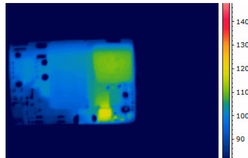
Figure 6. Thermal Image of CPT8A36N (8A output, 70C Ambient, 200lfm airflow, Vin = 48V, airflow from pin 3 to pin 1, Tmax = 118°C)
