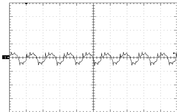
Figure 7. Output Voltage Ripple (50mV/div), time scale – 2uS/div. Vin=Vin_nom, full resistive Cout=1uF ceramic + 10uF Tantalum (see Fig 12)
