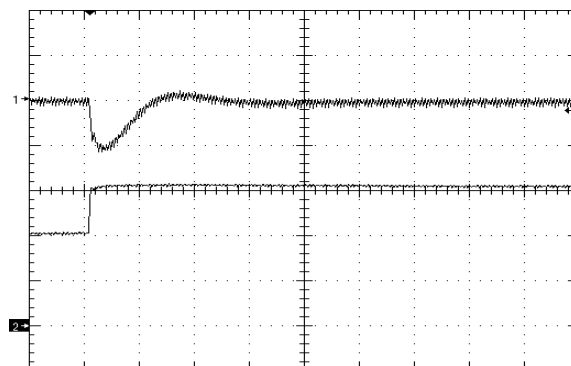
Figure 12. Load Transient Response (100mV/div), di/dt=2A/uS, 50% - 75% of full load, 330uF low ESR tantalum across output, time scale: 40uS/div.
