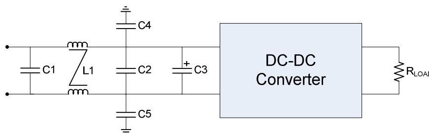
Figure 17. EMI Filter
