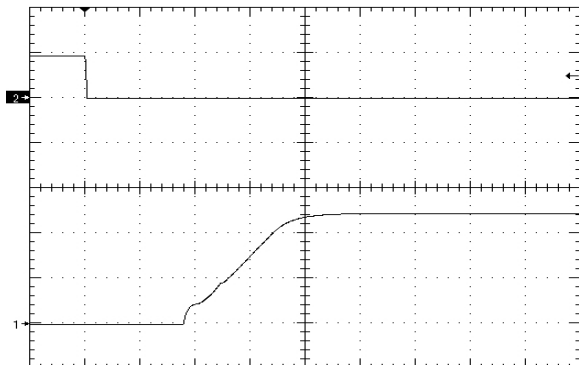
Figure 9. Startup Waveform (2V/div) via Enable Pin, time scale 4mS/div. Vin=Vin_nom, full resistive load (negative enable.)
