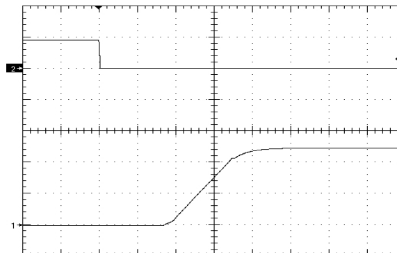
Figure 10. Startup Waveform (2V/div) via Enable Pin, time scale 4mS/div. Vin=Vin_nom, full resistive load + 4700uF (negative enable.)
