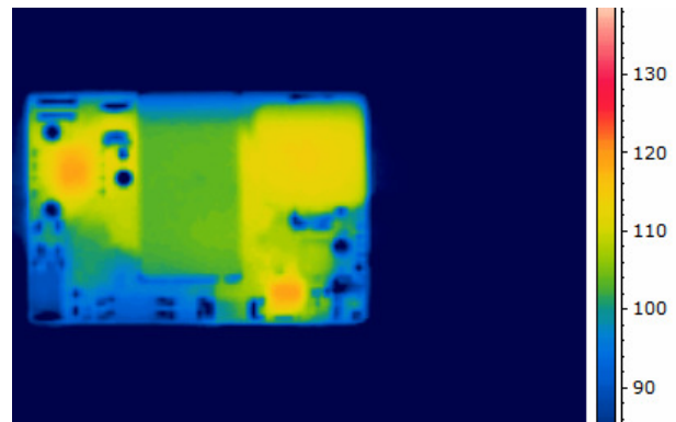
Figure 8. Thermal Image of CPT8A18 (8A output, 70C Ambient, 200lfm airflow, Vin = 18V, airflow from pin 3 to pin 1, T max = 117°C)
