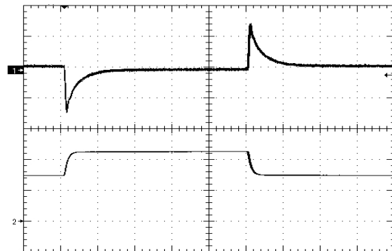
Figure 12. Load Transient Response (50mV/div), di/dt=0.1A/uS, 50% - 75% - 50% of full load, time scale: 200uS/div. Ch2 = 2A/div.
