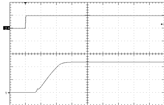
Figure 10. Startup Waveform via Enable Pin, time scale 10mS/div. Vin=Vin_nom, full resistive load + 2200uF, Ch1=Ch2=5V/div (positive enable.)
