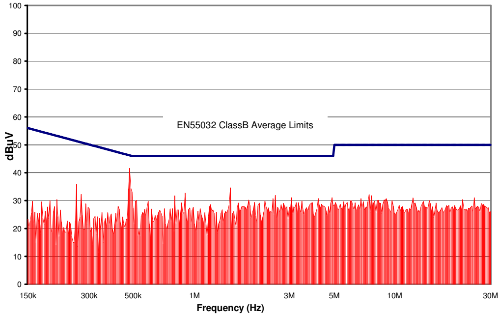
Figure 18. CPT6B36 Conducted Emissions using above specified input filter. Vin = 48V, Full Resistive Load
