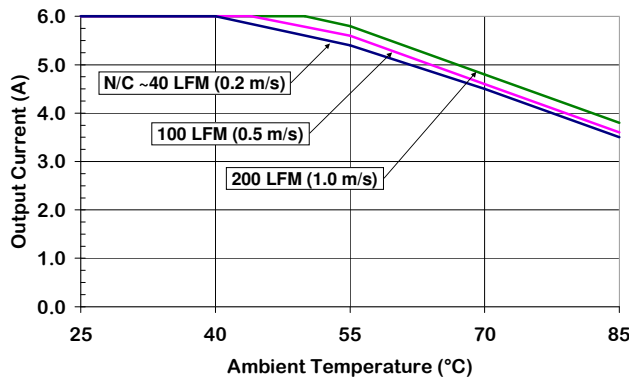
Figure 5. Output Current Derating vs Ambient Temperature & Airflow (air flowing from pin 3 to pin 1, Vin = 48 V, with baseplate.)
