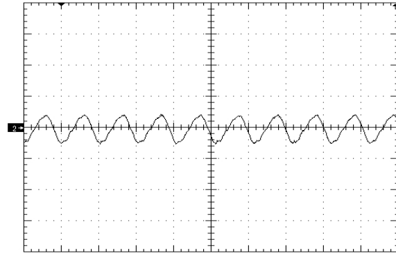
Figure 8. Input Reflected Ripple Current time scale - 2uS/div. Vin=Vin_nom, full resistive load (20mA/div)
