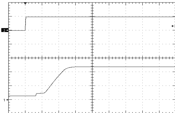
Figure 9. Startup Waveform via Enable Pin, time scale 10mS/div. Vin=Vin_nom, No Load, Co=0, Ch1=Ch2=5V/div (positive enable.)
