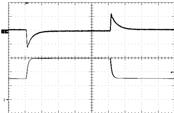
Figure 11. Load Transient Response (50mV/div), di/dt=0.1A/uS, 25% - 50% - 25% of full load, time scale: 200uS/div. Ch2 = 1A/div.
