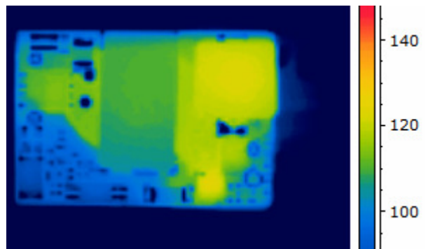
Figure 4. Thermal Image of CPT6A48 6A output, 85C Ambient, Natural Conv, Vin = 48V airflow from pin 3 to pin 1, T max = 120°C)
