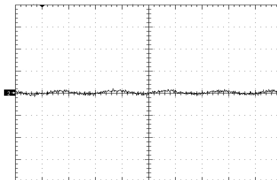
Figure 6. Input Reflected Ripple Current (10 mA/div) time scale - 1uS/div. Vin=Vin_nom, full resistive (see Fig 11)
