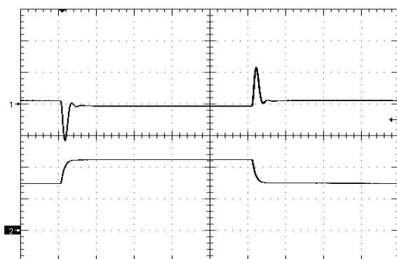
Figure 9. Load Transient Response di/dt=0.1A/uS, 50% - 75% - 50% of full load, time scale: 200uS/div Ch1=100mV/div, Ch2=2A/div
