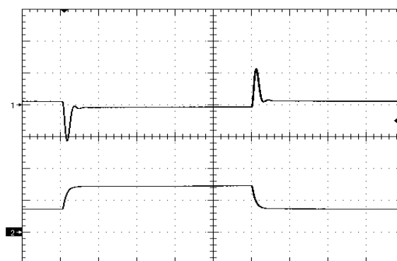
Figure 10. Load Transient Response (100mV/div), di/dt=0.1A/uS, 25% - 50% - 25% of full load, time scale: 200uS/div Ch1=100mV/div, Ch2=2A/div
