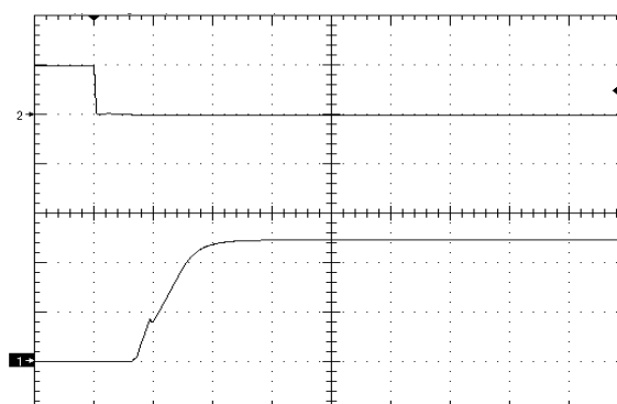
Figure 8. Startup Waveform via Enable Pin, time scale 10mS/div. Vin=Vin_nom, full resistive load + 4700uF, Ch1=2V/div, Ch2=5V/div
