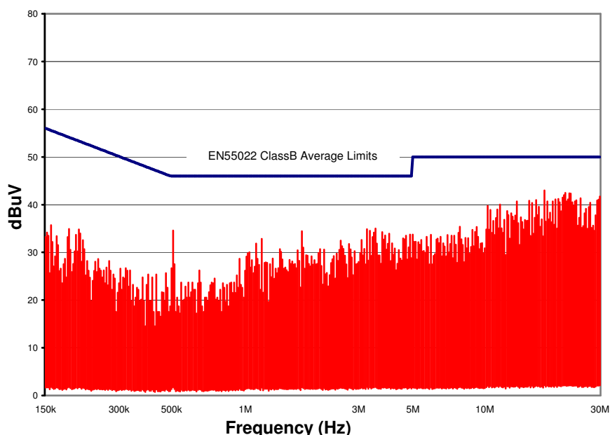
Figure 16. CPT6A48 Conducted Emissions using above specified input filter. Vin = 48V, Full Resistive Load
