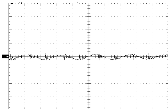
Figure 5. Output Voltage Ripple (20mV/div), time scale – 1uS/div. Vin=Vin_nom, full resistive Cout=1uF ceramic + 10uF ceramic (see Fig 12)
