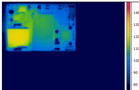
Figure 6. Thermal Image of CPT5C48 (5.5A output, 55C Ambient, 200lfm airflow, Vin = 48V, airflow from pin 1 to pin 3, T max = 125°C)
