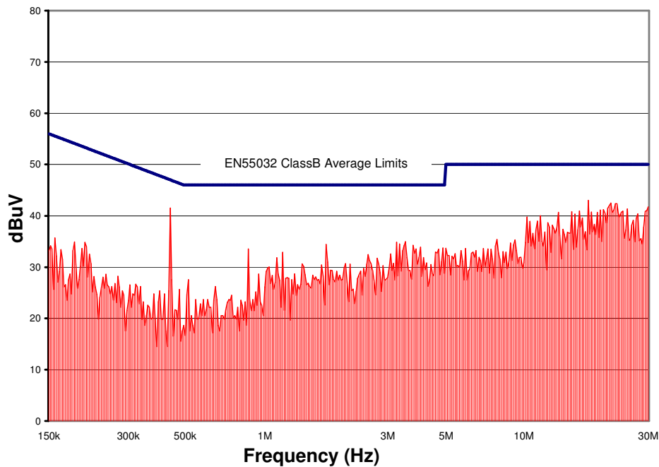
Figure 18. CPT5C48 Conducted Emissions using above specified input filter. Vin = 48V, Full Resistive Load
