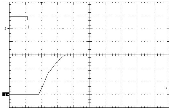
Figure 10. Startup Waveform via Enable Pin (5V/div), time scale 10mS/div. Vin=Vin_nom, full resistive load + 1000uF (negative enable.)
