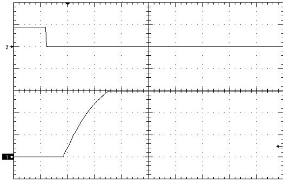
Figure 9. Startup Waveform via Enable Pin (5V/div), time scale 10mS/div. Vin=Vin_nom, full resistive load (negative enable.)
