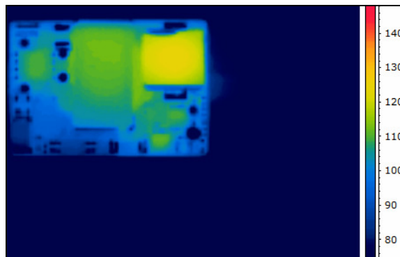
Figure 4. Thermal Image of CPT5C48 (5.5A output, 55C Ambient, 200lfm airflow, Vin = 48V, airflow from pin 3 to pin 1, T max = 124°C)
