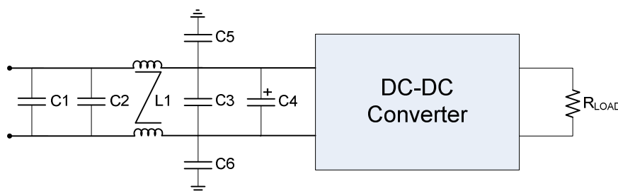
Figure 15. EMI Filter
