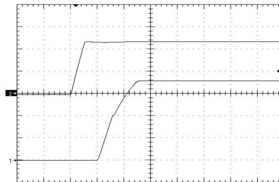
Figure 8. Startup Waveform via Line Voltage, time scale 10mS/div. Vin=Vin_nom, full res. load + 820uF, negative enbl, Ch1=5V/div, Ch2=20V/div
