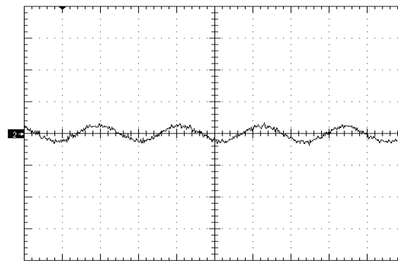
Figure 6. Input Reflected Ripple Current (10mA/div) time scale - 1uS/div. Vin=Vin_nom, full resistive.
