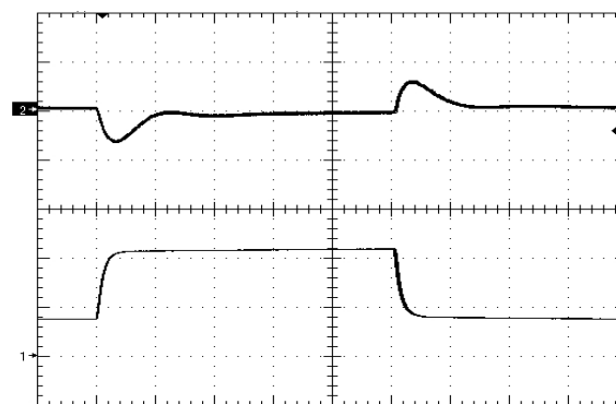
Figure 10. Load Transient Response (100mV/div), di/dt=0.1A/uS, 25% - 75% - 25% of full load + 820uF time scale: 200uS/div
