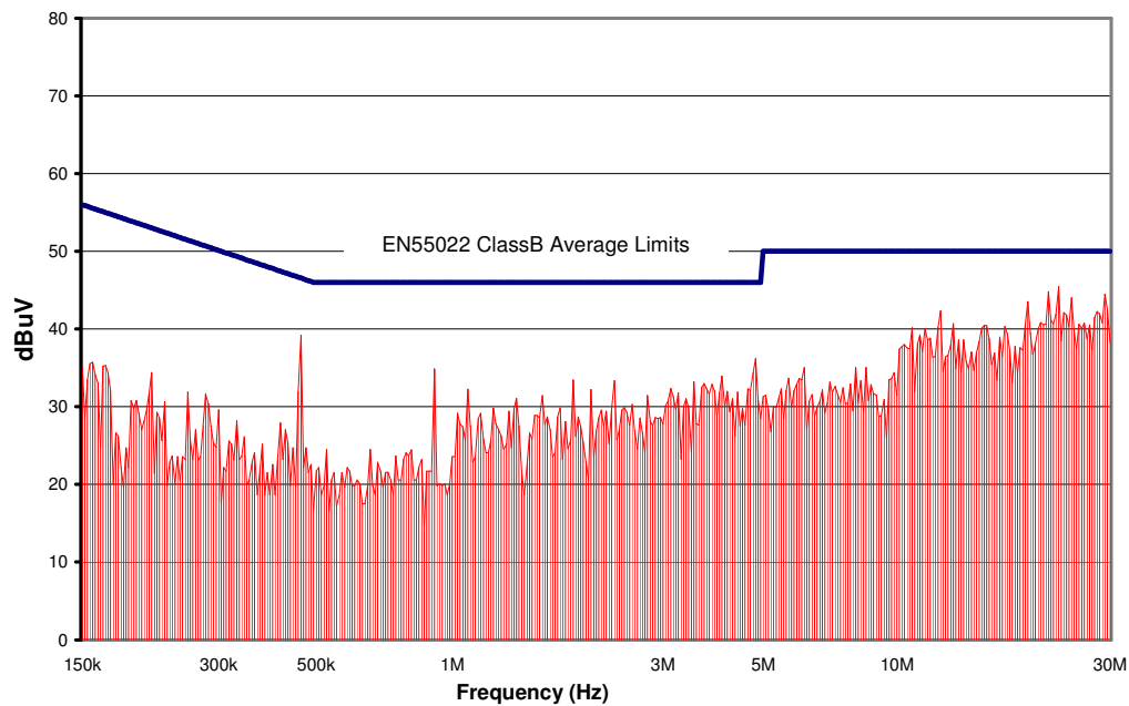
Figure 16. CPT3L48 Conducted Emissions using above specified input filter, Vin = 48V, Full Resistive Load
