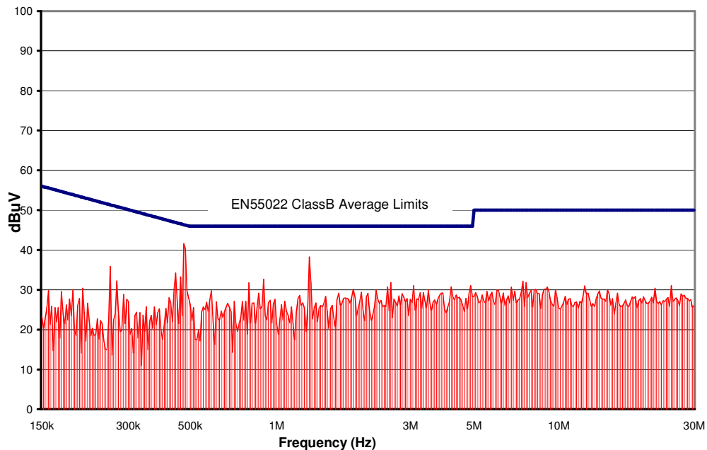
Figure 17. CPT2D36 Conducted Emissions using above specified input filter. Vin = 48V, Full Resistive Load
