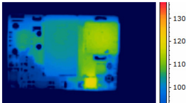
Figure 5. Thermal Image of CPT2D36 2A output, 55C Ambient, 200 LFM airflow Vin = 48V, airflow from pin 3 to pin 1, T max = 121 °C)
