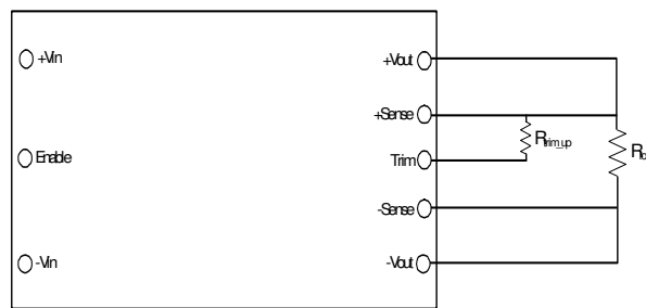
Figure 14. Trim UP circuit configuration
