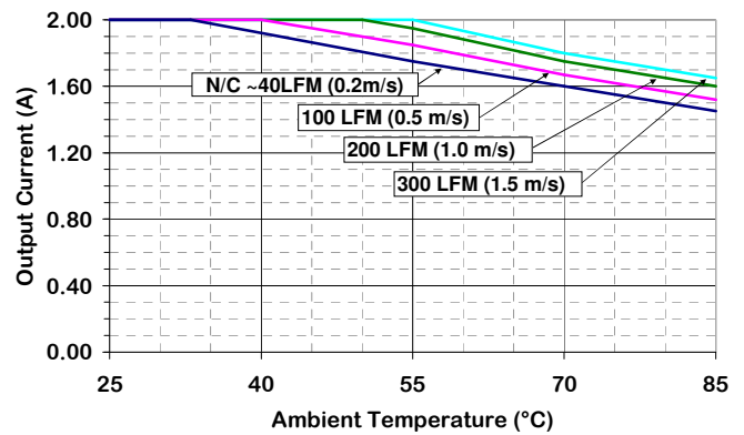
Figure 4. Output Current Derating vs Ambient Temperature & Airflow (converter mounted vertically with air flowing from pin 3 to pin 1, Vin = 24 Volts)
