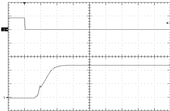
Figure 7. Startup Waveform via Enable Pin, time scale 10mS/div. Vin=Vin_nom, full load Ch1=1V/div, Ch2=5V/div
