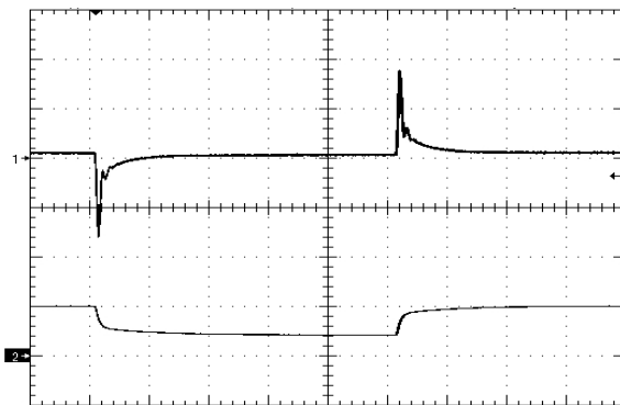
Figure 9. Load Transient Response (50mV/div), di/dt=0.1A/uS, 50% - 25% - 50% of full load, time scale: 200uS/div
