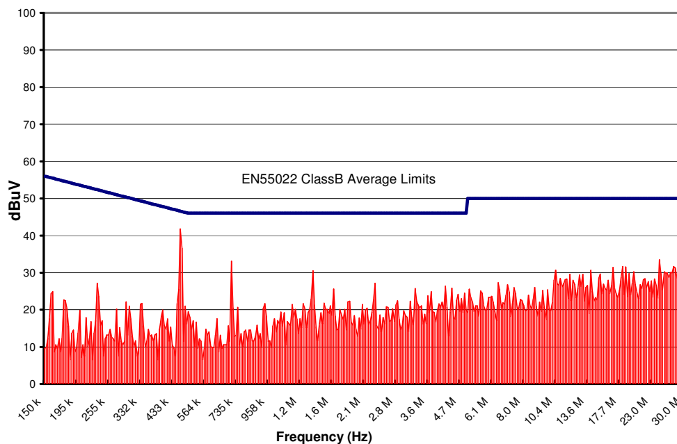
Figure 17. CPT20F48N Conducted Emissions using above specified input filter. Vin = 48V, Full Resistive Load
