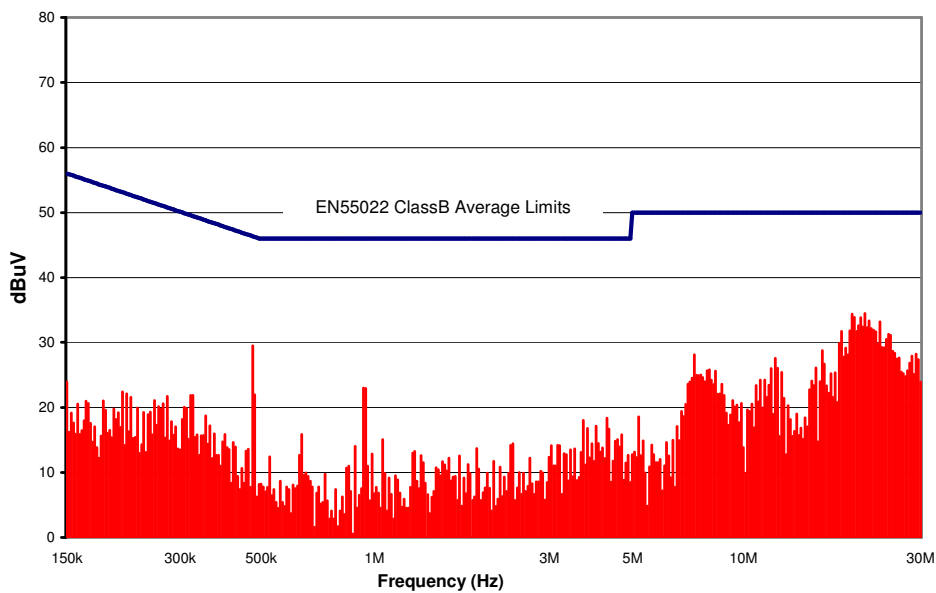
Figure 19. CPT15F18 Conducted Emissions using above specified input filter. Vin = 24V, Full Resistive Load (12Vin - subtract 2dB from peaks)
