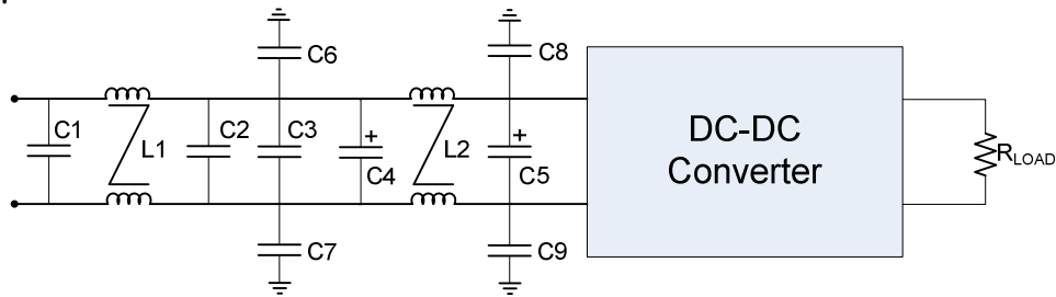
Figure 18. EMI Filter
