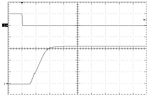
Figure 10. Startup Waveform (1V/div) via Enable Pin, time scale 10mS/div. Vin=Vin_nom, full resistive load + 10000uF (negative enable.) Ch2=5V/div
