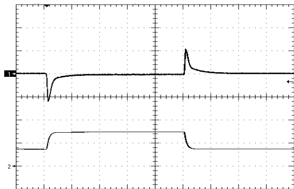
Figure 12. Load Transient Response (50mV/div), di/dt=0.1A/uS, 25% - 50% - 25% of full load, time scale: 200uS/div.
