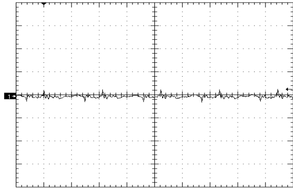
Figure 8. Output Voltage Ripple (50mV/div), time scale - 1uS/div. Vin=Vin_nom, full resistive Cout=1uF ceramic + 100uF Ceramic (see Fig 15)
