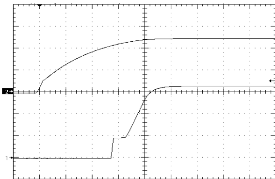
Figure 11. Waveform (1V/div) via Line Voltage, time scale 10mS/div. Vin=12V, no load Ch1=1V/div, Ch2=5V/div
