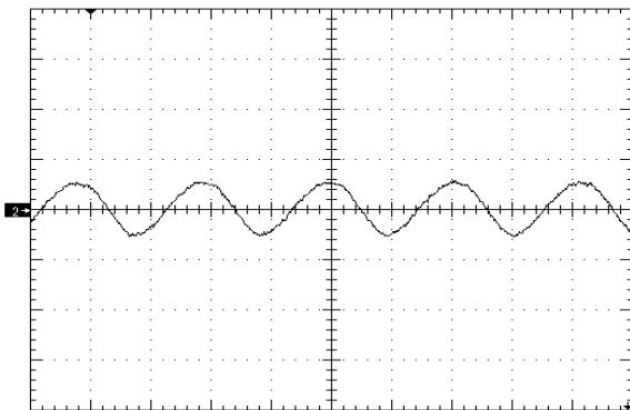
Figure 9. Input Reflected Ripple Current (20mA/div) time scale - 2uS/div. Vin=Vin_nom, full resistive
