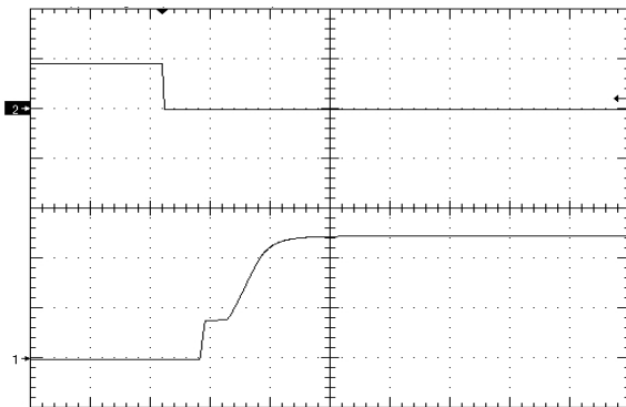
Figure 8. Startup Waveform (2V/div) via Enable Pin, time scale 10mS/div. Vin=Vin_nom, no load Negative enable, Ch2=5V/div
