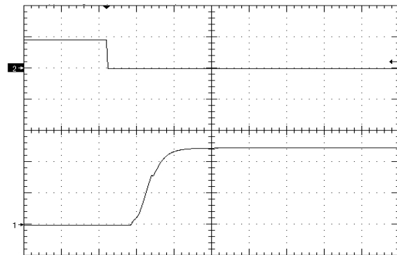
Figure 9. Startup Waveform (2V/div) via Enable Pin, time scale 10mS/div. Vin=Vin_nom, full resistive load + 4700uF, Negative enable, Ch2=5V/div
