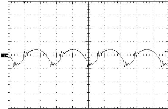
Figure 6. Output Voltage Ripple (50mV/div), time scale - 1uS/div. Vin=Vin_nom, full resistive Cout=1uF ceramic + 10uF Tantalum (see Fig 12)
