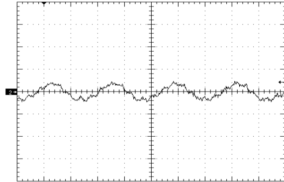
Figure 7. Input Reflected Ripple Current (10 mA/div) time scale - 1uS/div. Vin=Vin_nom, full resistive (see Fig 11)
