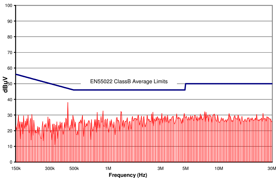
Figure 16. CPT14A36 Conducted Emissions using above specified input filter. Vin = 48V, Full Resistive Load
