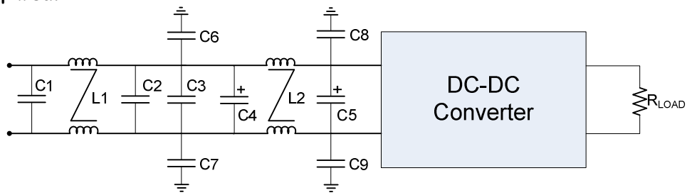
Figure 15. EMI Filter
