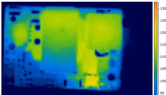
Figure 5. Thermal Image of CPT14A36 14A output, 55C Ambient, 200 LFM airflow Vin = 48V, airflow from pin 3 to pin 1, Tmax = 123°C)
