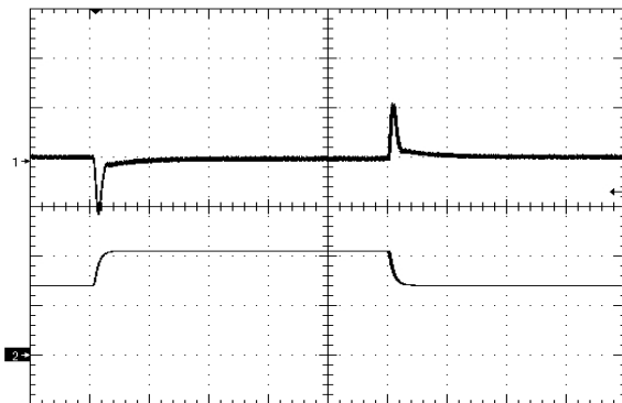
Figure 10. Load Transient Response (100mV/div), di/dt=0.1A/uS, 50% - 75% - 50% of full load, time scale: 200µS/div. Ch2=5A/div
