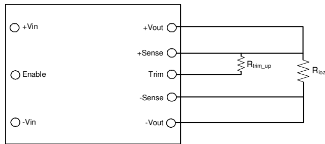
Figure 14. Trim UP circuit configuration
