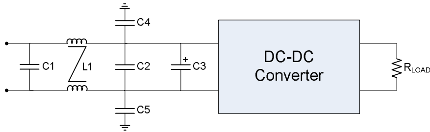
Figure 16. EMI Filter
