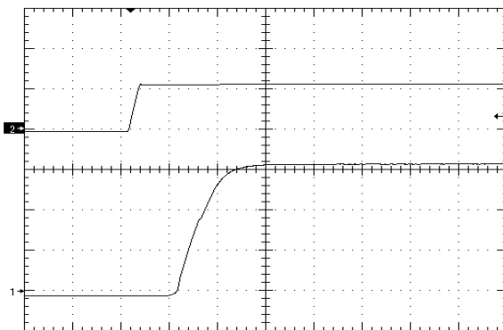
Figure 11. Waveform (1V/div) via Line Voltage, time scale 10mS/div. Vin=24Vin, full resistive load + 10000uF across output.
