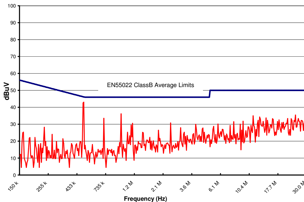
Figure 18. CPT12F36 Conducted Emissions using above specified input filter. Vin = 48V, Full Resistive Load (24Vin - subtract 2dB from peaks)
