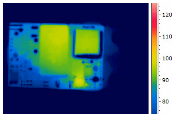
Figure 6. Thermal Image of CPT12F36N (12A output, 55C Ambient, 200lfm airflow, Vin = 48V, airflow from pin 3 to pin 1, Tmax = 98°C)
