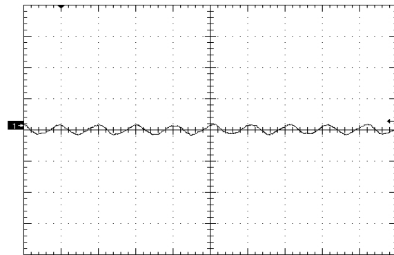
Figure 8. Input Reflected Ripple Current (5mA/div) time scale - 2uS/div. Vin=Vin_nom, full resistive
