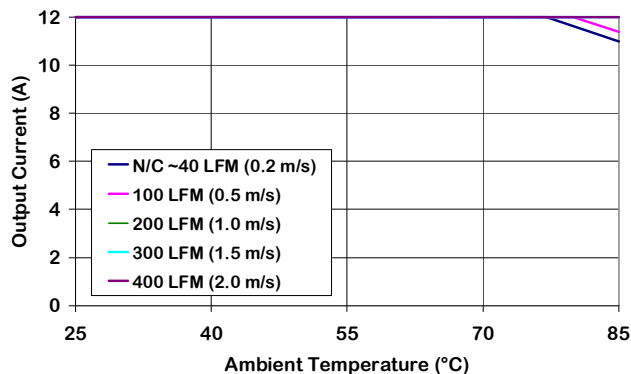
Figure 6. Output Current Derating vs Ambient Temperature & Airflow (converter mounted vertically with air flowing from pin 3 to pin 1, Vin = 24 V.)
