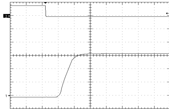
Figure 12. Startup Waveform (1V/div) via Enable Pin, time scale 10mS/div. Vin=Vin_nom, full resistive load + 10000uF (negative enable.)
