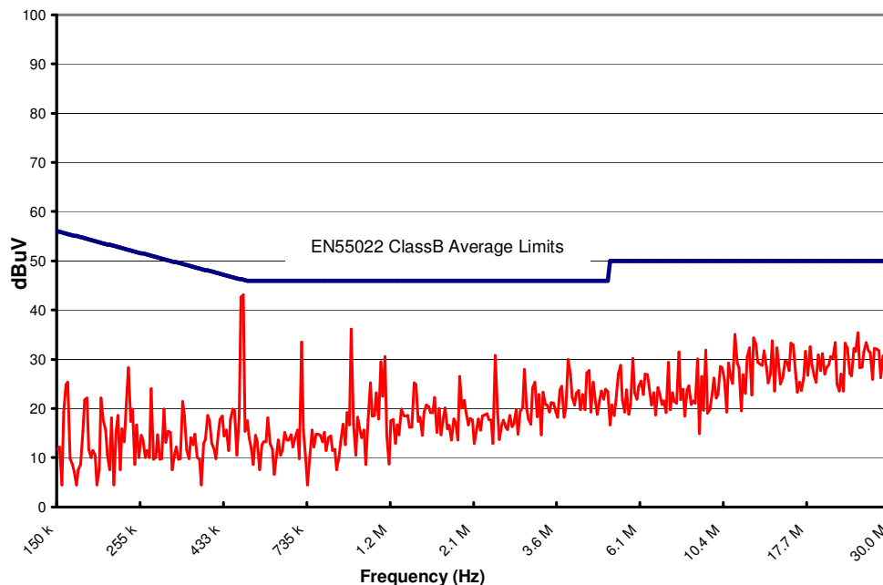
Figure 18. CPT12F36N Conducted Emissions using above specified input filter. Vin = 48V, Full Resistive Load (24Vin - subtract 2dB from peaks)
