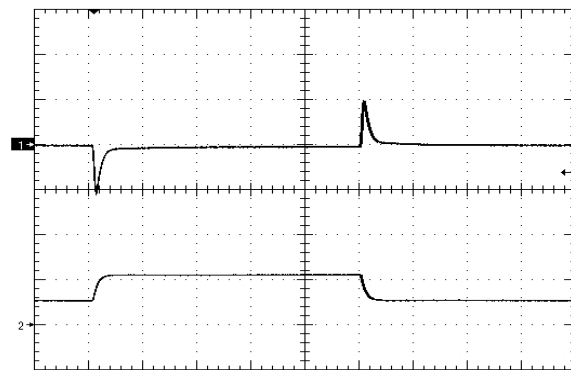
Figure 14. Load Transient Response (100mV/div), di/dt=0.1A/uS, 25% - 50% - 25% of full load, time scale: 200uS/div.
