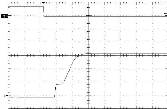
Figure 11. Startup Waveform (1V/div) via Enable Pin, time scale 10mS/div. Vin=24Vin, no load, no capacitance across output.
