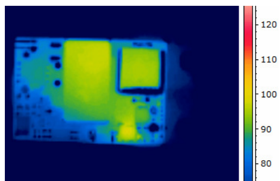
Figure 8. Thermal Image of CPT12F36N (12A output, 55C Ambient, 200lfm airflow, Vin = 48V, airflow from pin 3 to pin 1, Tmax = 98°C)
