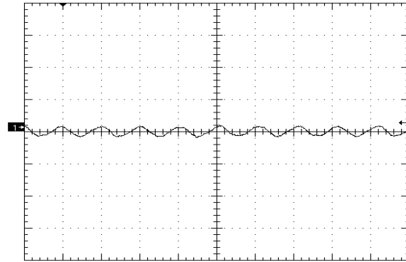
Figure 10. Input Reflected Ripple Current (5mA/div) time scale - 2uS/div. Vin=Vin_nom, full resistive
