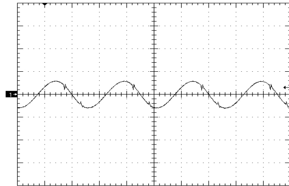
Figure 8. Output Voltage Ripple (50mV/div), time scale - 1uS/div. Vin=Vin_nom, full resistive Cout=.1uF ceramic + 22uF Ceramic (see Fig 15)
