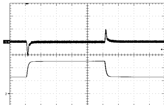
Figure 12. Load Transient Response (100mV/div), di/dt=0.1A/uS, 25% - 50% - 25% of full load, time scale: 200uS/div. Ch2 = 2A/div
