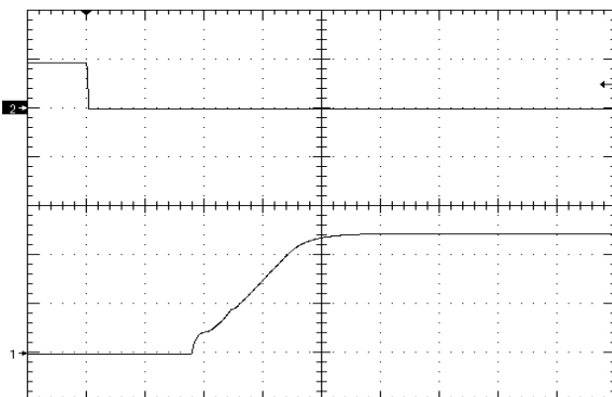
Figure 11. Waveform (2V/div) via Enable Pin, time scale 5mS/div. Vin=Vin_nom, full resistive load (negative enable.) Ch2=5V/div
