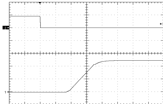
Figure 10. Startup Waveform (2V/div) via Enable Pin, time scale 5mS/div. Vin=Vin_nom, full resistive load + 4700uF (negative enable.) Ch2=5V/div
