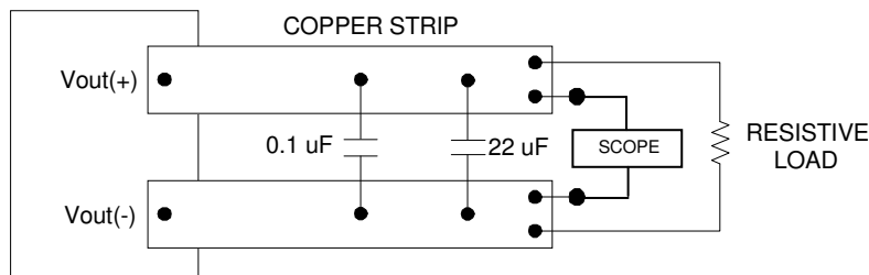
Figure 14. Peak-to-Peak Output Noise Measurement Test Setup.
