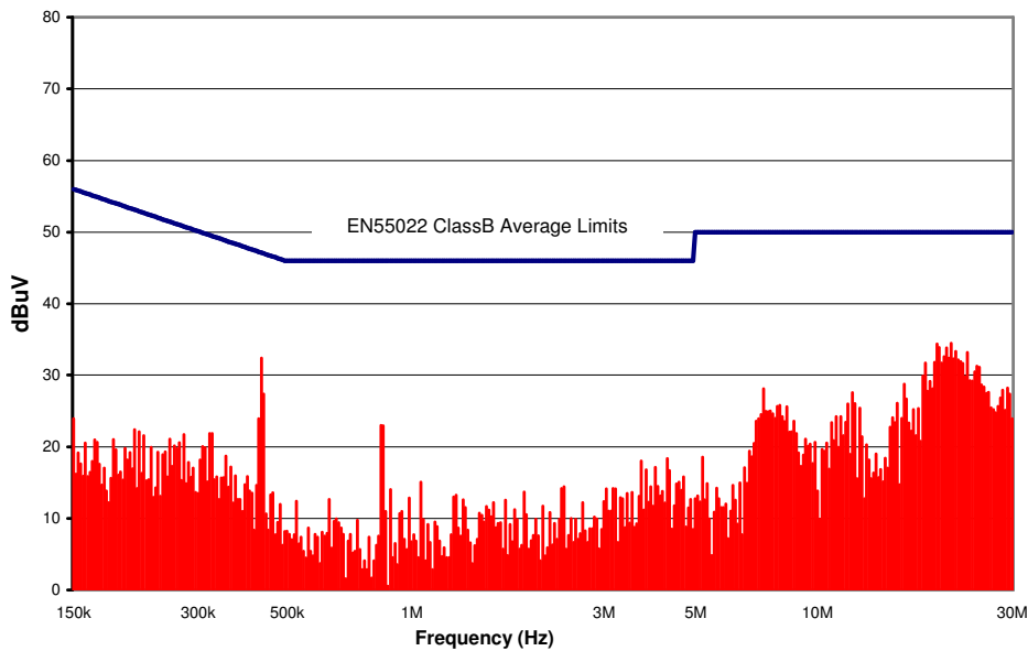
Figure 19. CPT10A18 Conducted Emissions using above specified input filter. Vin = 24V, Full Resistive Load (12Vin - subtract 2dB from peaks)
