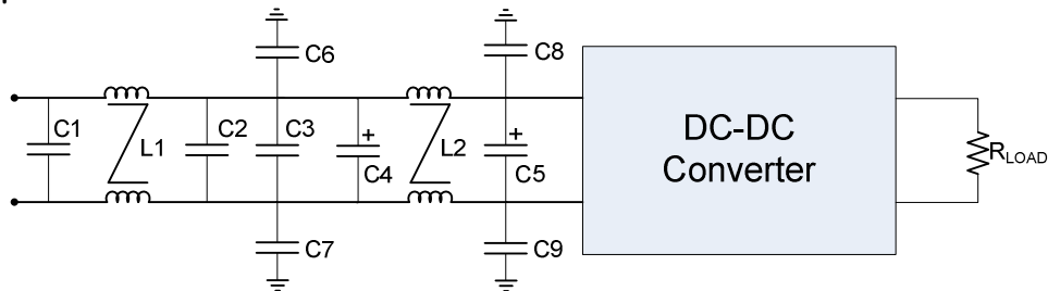
Figure 16. EMI Filter
