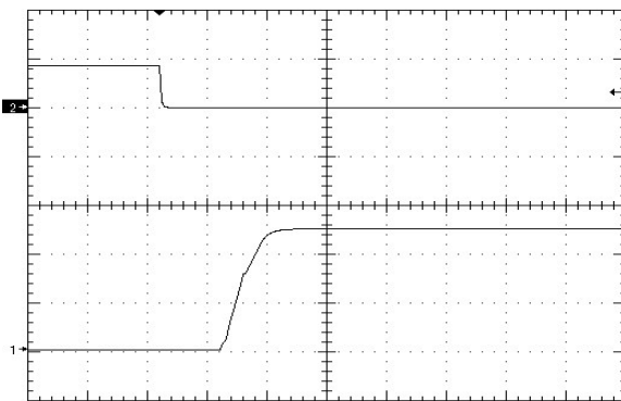
Figure 9. Waveform (2V/div) via Enable Pin, time scale 10mS/div. Vin=Vin_nom, full resistive load (negative enable.) Ch2=5V/div
