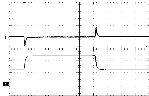
Figure 10. Load Transient Response (50mV/div), di/dt=0.1A/uS, 25% - 50% - 25% of full load, time scale: 200uS/div. Ch2=2A/div
