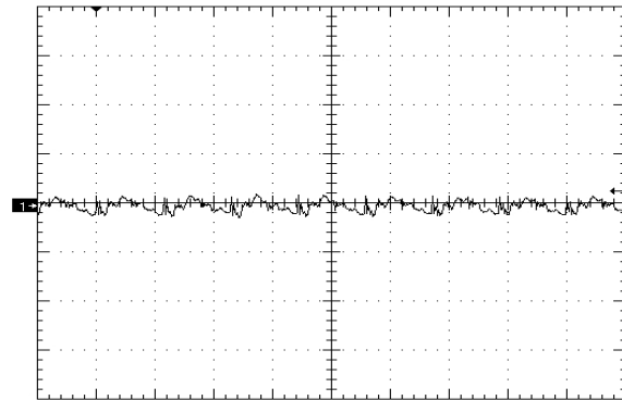
Figure 6. Output Voltage Ripple (50mV/div), time scale - 2uS/div. Vin=Vin_nom, full resistive Cout=1uF ceramic + 47uF Ceramic (see Fig 13)
