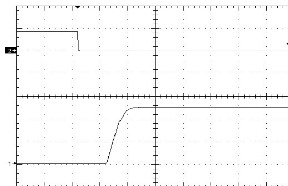
Figure 8. Startup Waveform (2V/div) via Enable Pin, time scale 10mS/div. Vin=Vin_nom, full resistive load + 4700uF (negative enable.) Ch2=5V/div
