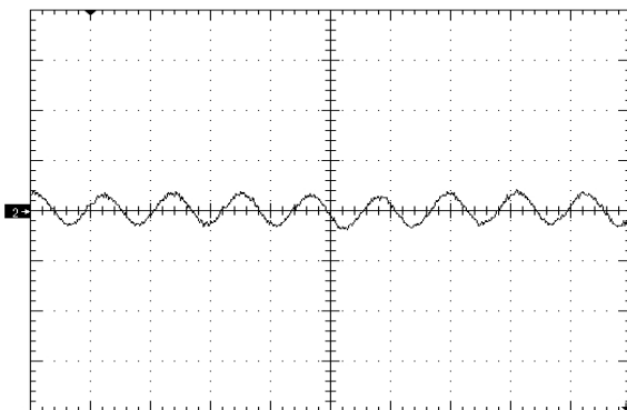
Figure 7. Input Reflected Ripple Current (10mA/div) time scale - 2uS/div. Vin=Vin_nom, full resistive
