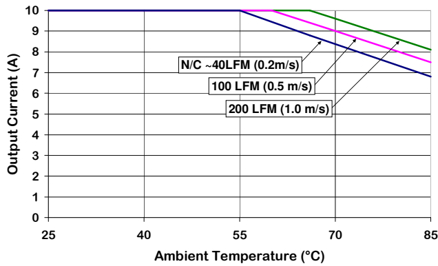
Figure 3. Output Current Derating vs Ambient Temperature & Airflow (converter mounted vertically with air flowing from pin 3 to pin 1, Vin = 12 V.) (EST.)
