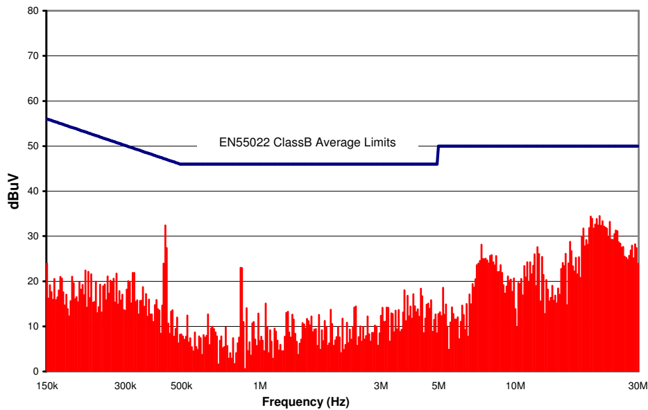
Figure 17. CPT10A12 Conducted Emissions using above specified input filter. Vin = 12V, Full Resistive Load
