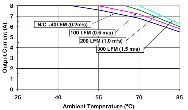
Figure 6. Output Current Derating vs Ambient Temperature & Airflow (air flowing from pin 3 to pin 1, Vin = 12 V, with baseplate)
