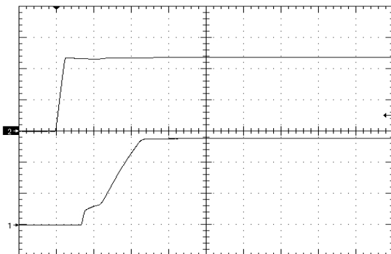
Figure 7. Startup Waveform via Line Voltage, time scale 10mS/div. Vin=Vin_nom, no load Ch1,Ch2=10V/div
