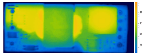
Thermal Image of module @ 24Vin, 300LFM & 40C
