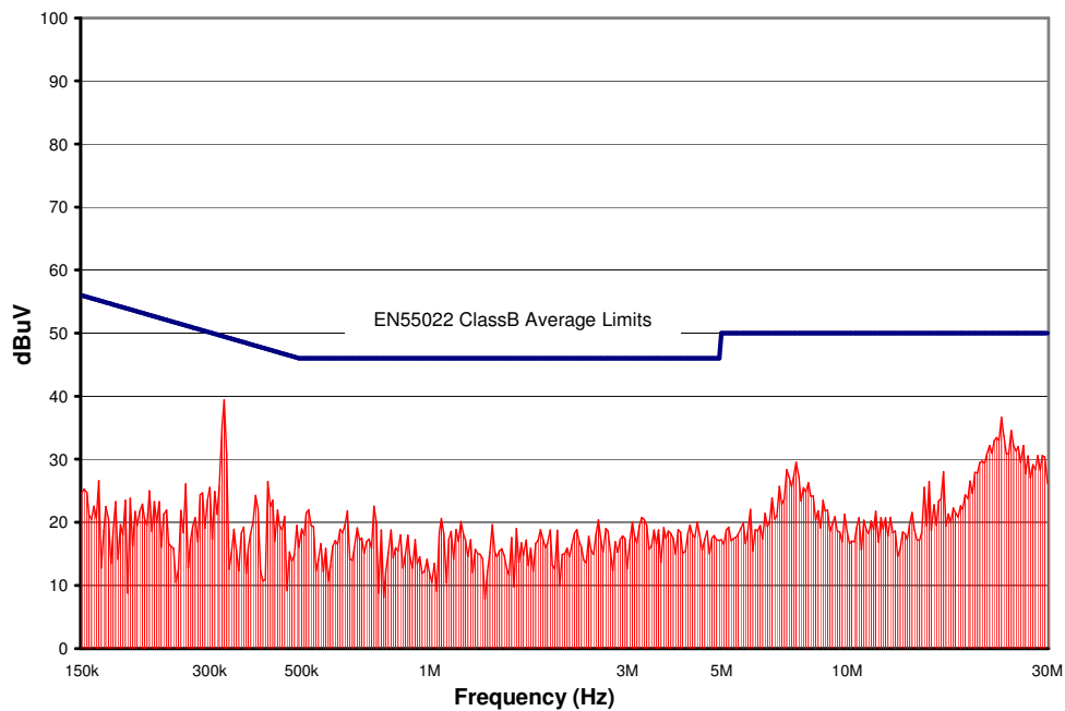
Figure 16. CPE6R24 Conducted Emissions using above specified input filter, Vin = 48V, Full Resistive Load
