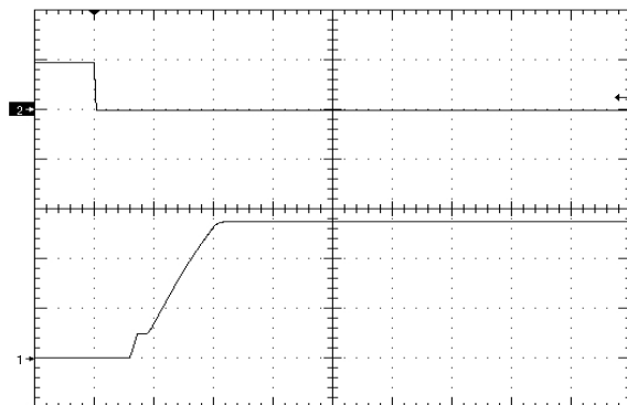
Figure 8. Startup Waveform via Enable Pin, time scale 10mS/div. Vin=Vin_nom, full resistive load + 1000uF. Ch1=5V/div,Ch2=10V/div
