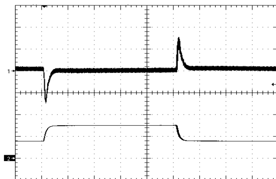
Figure 10. Load Transient Response (100mV/div), di/dt=0.1A/uS, 25% - 50% - 25% of full load, time scale: 200uS/div. Ch2=2A/div
