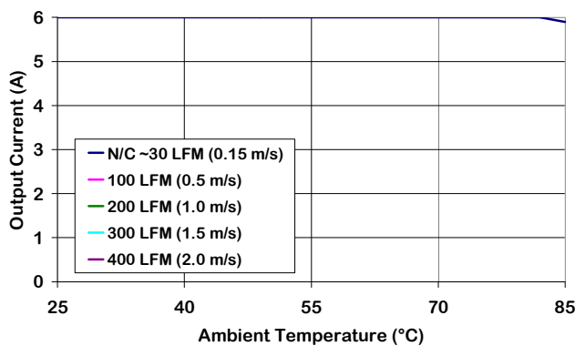
Figure 5. Output Current Derating vs Ambient Temperature & Airflow (converter mounted vertically with air flowing from Vout to Vin, Vin = 48 V.)
