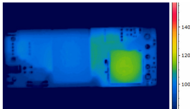
Figure 6. Thermal Image of CPE6B48 (6A output, 85C Ambient, 200lfm airflow, Vin = 48V, airflow from pin 3 to pin 1, T max = 114°C)
