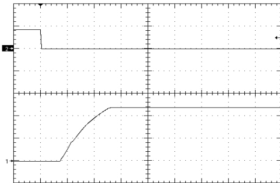
Figure 9. Startup Waveform via Enable Pin (5V/div), time scale 10mS/div. Vin=Vin_nom, full resistive load (negative enable.)
