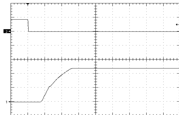
Figure 10. Startup Waveform via Enable Pin (5V/div), time scale 10mS/div. Vin=Vin_nom, full resistive load + 3300uF (negative enable.)
