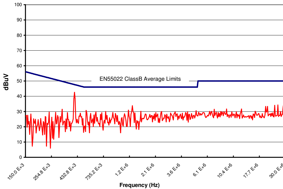
Figure 18. CPE6B48 Conducted Emissions using above specified input filter. Vin = 48V, Full Resistive Load
