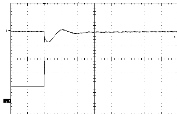
Figure 12. Load Transient Response (100mV/div), di/dt=3.0A/uS, 25% - 75% of full load, 2000uF Oscon low ESR across output, time scale: 200uS/div.
