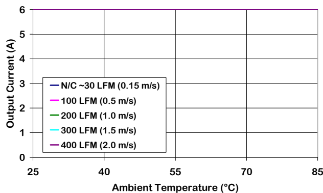
Figure 4. Output Current Derating vs Ambient Temperature & Airflow (converter mounted vertically with air flowing from pin 1 to pin 3, Vin = 48 V.)
