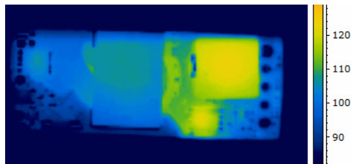
Figure 6. Thermal Image of CPE4D36 (4A output, 55C Ambient, 200lfm airflow, Vin = 48V, airflow from pin 3 to pin 1, T max = 122°C)
