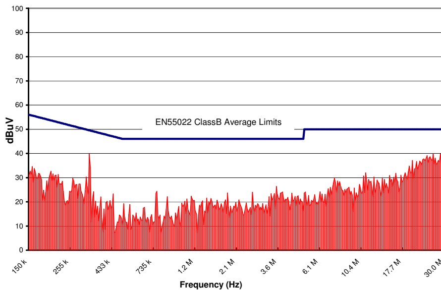
Figure 18. CPE4D36 Conducted Emissions using above specified input filter, Vin = 48V, Full Resistive Load
