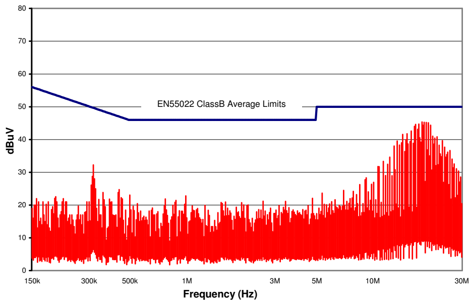
Figure 18. CPE4D24 Conducted Emissions using above specified input filter, Vin = 24V, Full Resistive Load
