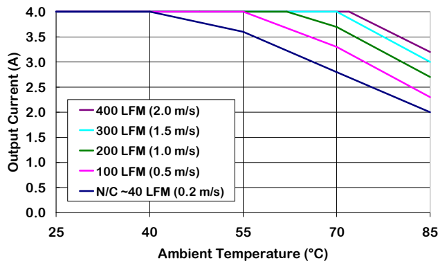
Figure 5. Output Current Derating vs Ambient Temperature & Airflow (converter mounted vertically with air flowing from pin 3 to pin 1, Vin = 30 V.)
