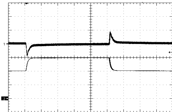
Figure 11. Load Transient Response (100mV/div), di/dt=0.05A/uS, 50% - 75% - 50% of full load, Ch2=1A/div, time scale: 200uS/div.
