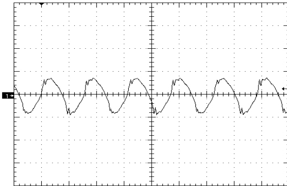
Figure 7. Output Voltage Ripple (50mV/div), time scale – 2S/div. Vin=Vin_nom, full resistive.
