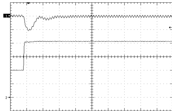
Figure 12. Load Transient Response (500mV/div), di/dt=1A/uS, 50% - 100% of full load, Ch2=1A/div, time scale: 20uS/div
