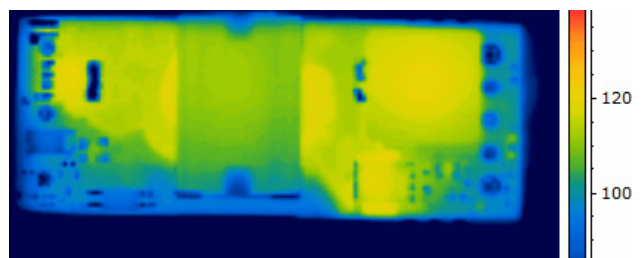
Figure 6. Thermal Image of CPE4D18 (4A output, 55C Ambient, 200lfm airflow, Vin = 24V, airflow from pin 3 to pin 1, T max = 122°C)
