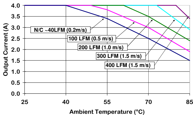
Figure 5. Output Current Derating vs Ambient Temperature & Airflow (air flowing from pin 3 to to pin 1, Vin = 24 V with baseplate)
