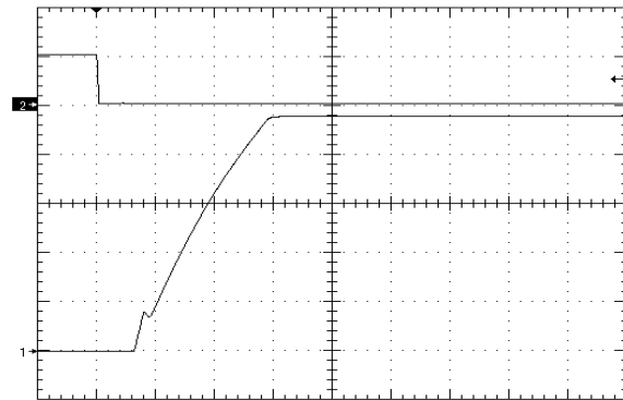
Figure 10. Startup Waveform via Enable Pin, time scale 10mS/div. Vin=Vin_nom, full resistive load + 1000uF (neg en) Ch1=5V/div, Ch2=5V/div
