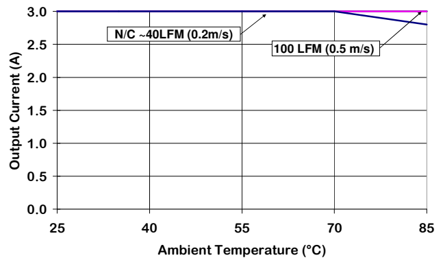
Figure 4. Output Current Derating vs Ambient Temperature & Airflow (air flowing from pin 3 to to pin 1, Vin = 48 V without baseplate)
