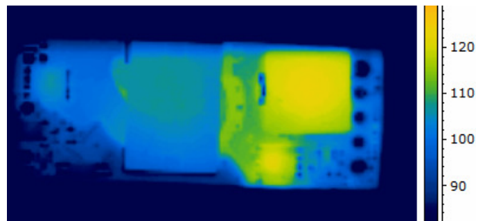
Figure 6. Thermal Image of CPE3D36 (3A output, 85C Ambient, 100lfm airflow, Vin = 48V, airflow from pin 3 to pin 1, T max = 122°C)
