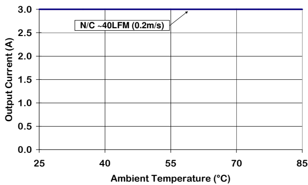
Figure 5. Output Current Derating vs Ambient Temperature & Airflow (air flowing from pin 3 to to pin 1, Vin = 24-48 V with baseplate)
