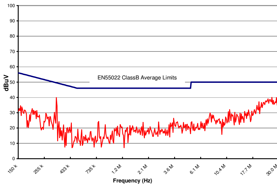
Figure 18. CPE3D36 Conducted Emissions using above specified input filter, Vin = 48V, Full Resistive Load
