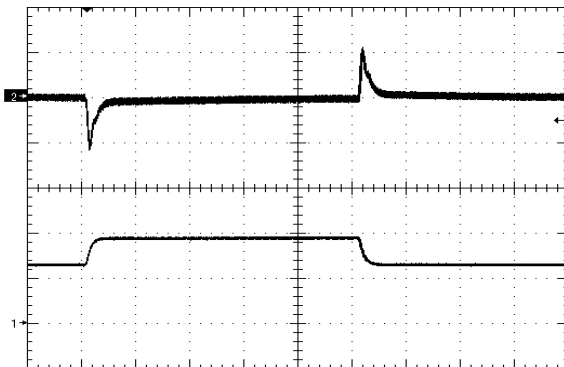
Figure 11. Load Transient Response (100mV/div), di/dt=0.05A/uS, 50% - 75% - 50% of full load, time scale: 200uS/div.
