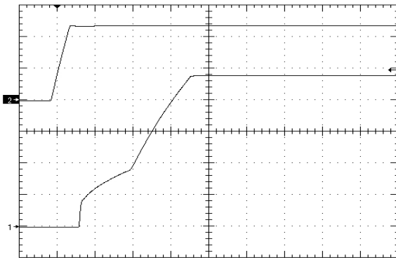
Figure 9. Startup Waveform via Line Voltage, time scale 10mS/div. Vin=Vin_nom, no load Ch1=5V/div, Ch2=20V/div
