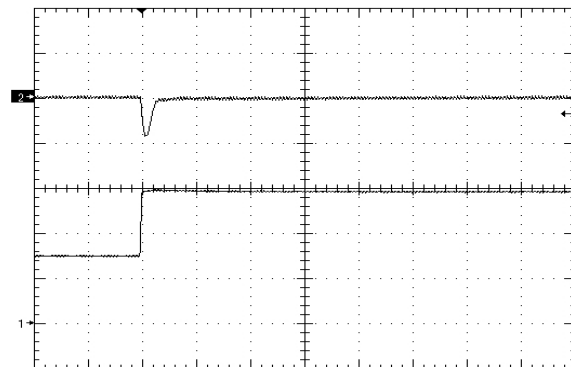
Figure 12. Load Transient Response (500mV/div), di/dt=1A/uS, 50% - 100% of full load, time scale: 100uS/div
