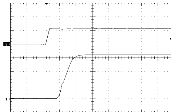
Figure 10. Startup Waveform via Enable Pin, time scale 10mS/div. Vin=48VDC, full resistive load + 4700uF, Ch1=1V/div, Ch2=5V/div
