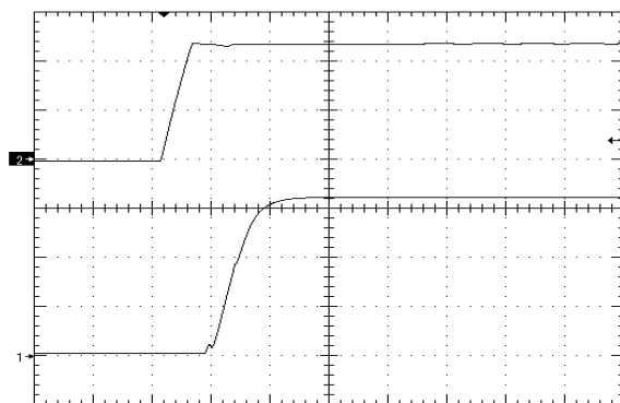
Figure 9. Startup Waveform via Line Voltage, time scale 10mS/div. Vin=48VDC, full resistive load + 4700uF, Ch1=1V/div, Ch2=20V/div
