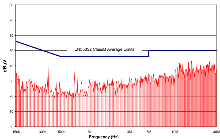
Figure 18. CPE30F48 Conducted Emissions using above specified input filter. Vin = 48V, Full Resistive Load
