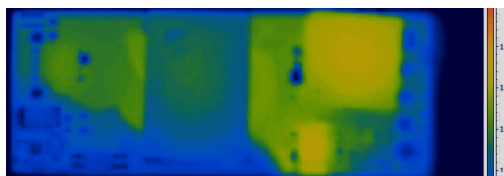
Thermal Image @ 48Vin, 30A, 200LFM & 55C
