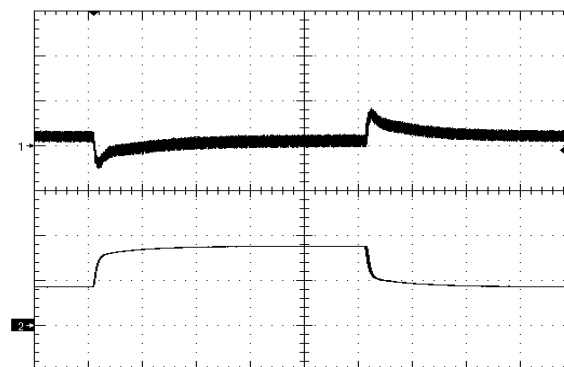
Figure 12. Load Transient Response (50mV/div), di/dt=0.2 A/uS, 25% - 50% - 25% of full load + 4700uF Ch2=10A/div, time scale: 200uS/div
