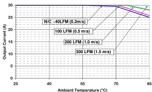
Figure 4. Output Current Derating vs Ambient Temperature & Airflow (air flowing from pin 3 to pin 1, Vin = 48 V, with baseplate)
