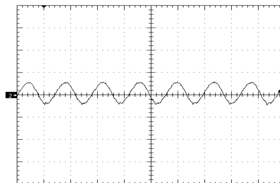
Figure 8. Input Reflected Ripple Current (20mA/div) time scale - 2uS/div. Vin=Vin_nom, full resistive
