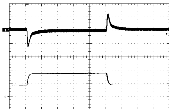
Figure 11. Load Transient Response (50mV/div), di/dt=0.2A/uS, 25% - 50% - 25% of full load, Ch2=10A/div, time scale: 200uS/div
