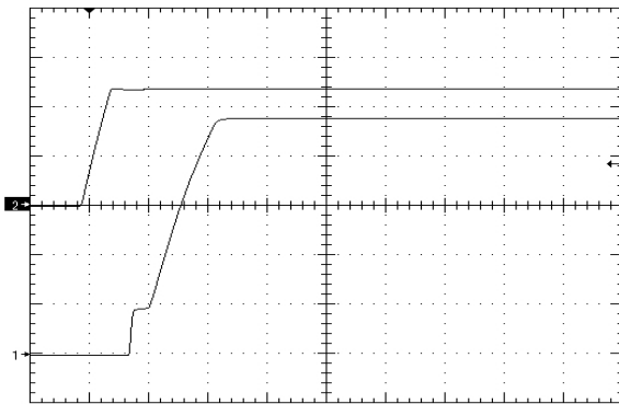
Figure 9. Startup Waveform via Line Voltage, time scale 10mS/div. Vin=Vin_nom, full resistive load (negative enable.) Ch1=5V/div, Ch2=20V/div
