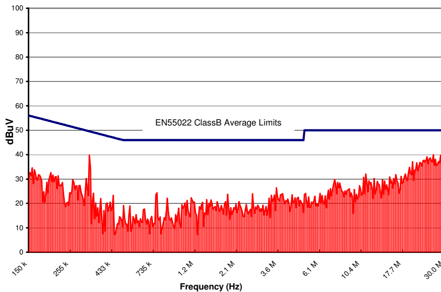
Figure 18. CPE2U96 Conducted Emissions using above specified input filter, Vin = 96V, Full Resistive Load
