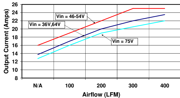
Figure 6. Current Derating vs Airflow & Line Voltage (converter mounted vertically with air flowing from pin 3 to pin 1, Tambient = 55C) with baseplate
