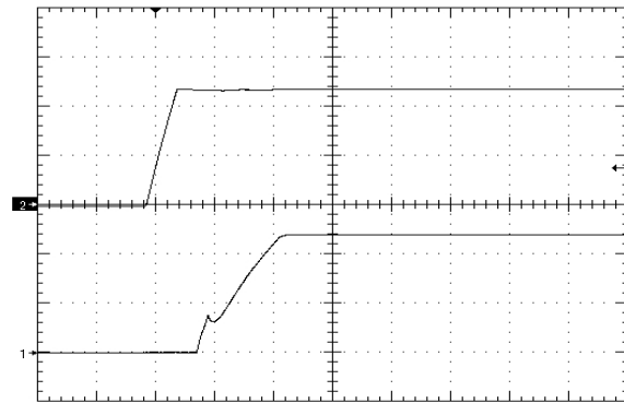
Figure 10. Startup Waveform via Enable Pin, time scale 10mS/div. Vin=Vin_nom, full resistive load (negative enable.) Ch1,Ch2=5V/div
