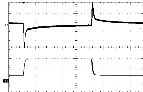
Figure 12. Load Transient Response (200mV/div), di/dt=0.2A/uS, 25% - 100% - 25% of full load, time scale: 200uS/div
