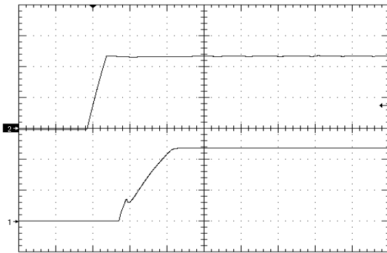
Figure 9. Startup Waveform via Line Voltage, time scale 10mS/div. Vin=Vin_nom, full resistive load Ch1=5V/div, Ch2=20V/div
