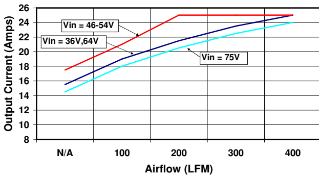
Figure 5. Output Current Derating vs Airflow & Line Voltage (converter mounted vertically with air flowing from pin 3 to pin 1, Tambient = 40C) with baseplate
