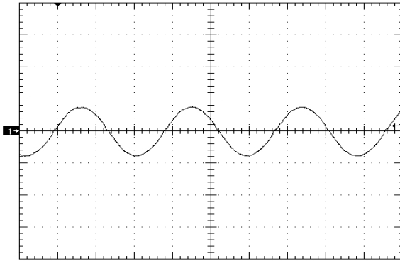
Figure 7. Output Voltage Ripple (100mV/div), time scale – 1uS/div. Vin=Vin_nom, full resistive.
