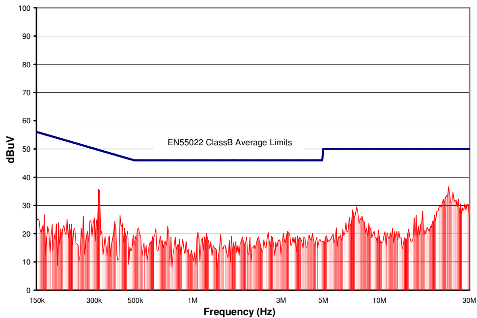
Figure 16. CPE25A24 Conducted Emissions using above specified input filter, Vin = 24V, Full Resistive Load
