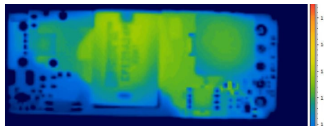
Thermal Image of module @ 24Vin, 200LFM & 25C
