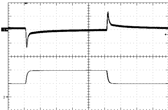
Figure 9. Load Transient Response (200mV/div), di/dt=0.1A/uS, 50% - 100% - 50% of full load, time scale: 200uS/div.
