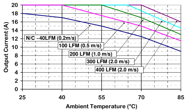
Figure 4. Current Derating vs Ambient Temperature & Airflow (converter mounted vertically with air flowing from pin 3 to pin 1, Vin = 48 V) with baseplate
