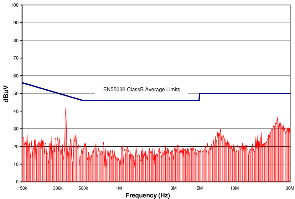
Figure 16. CPE20B48 Conducted Emissions using above specified input filter, Vin = 48V, Full Resistive Load
