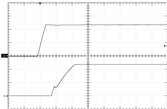
Figure 7. Startup Waveform via Line Voltage, time scale 10mS/div. Vin=Vin_nom, full resistive load Ch1=5V/div, Ch2=20V/div
