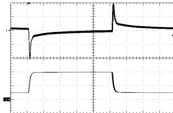
Figure 10. Load Transient Response (200mV/div), di/dt=0.2A/uS, 25% - 100% - 25% of full load, time scale: 200uS/div
