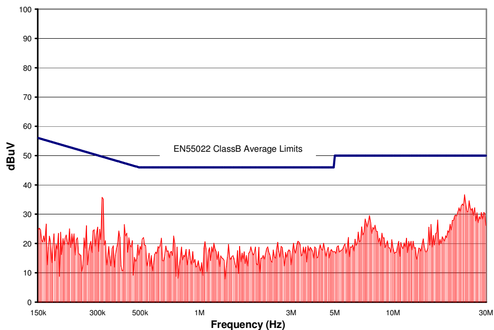
Figure 16. CPE20A48 Conducted Emissions using above specified input filter, Vin = 48V, Full Resistive Load
