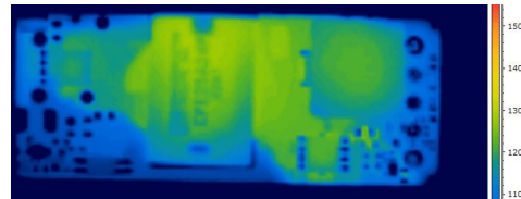
Thermal Image of module @ 48Vin, 100LFM & 65C
