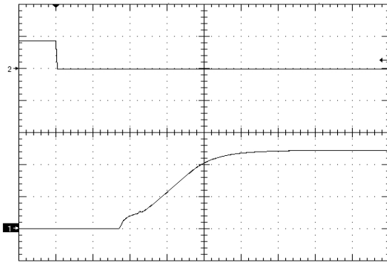
Figure 9. Startup Waveform via Enable Pin, time scale 4mS/div. Vin=Vin_nom, full resistive load (negative enable.) Ch1=2V/div,Ch2=5V/div
