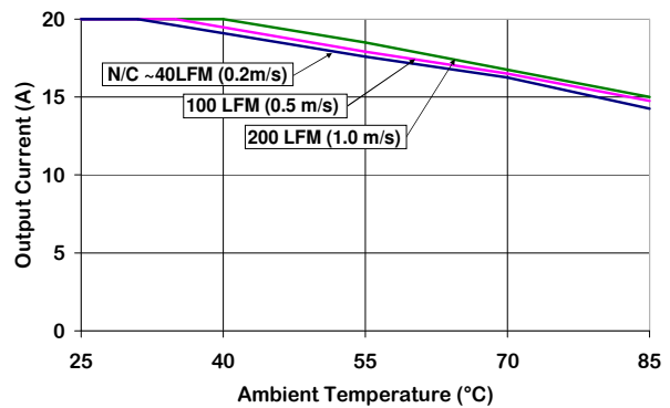
Figure 6. Output Current Derating vs Ambient Temperature & Airflow (air flowing from pin 3 to with pin 1, Vin = 12 V, with baseplate)
