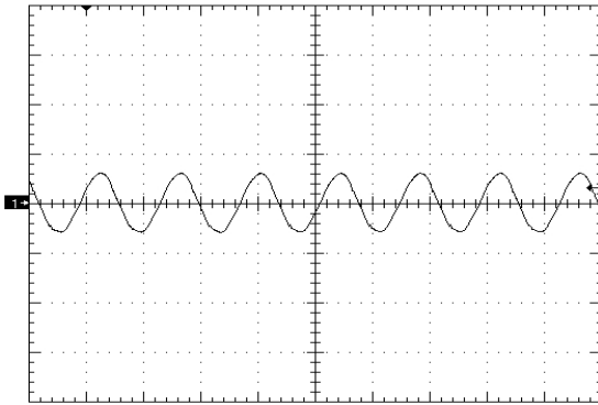
Figure 7. Output Voltage Ripple (50mV/div), time scale – 2uS/div. Vin=Vin_nom, full resistive.
