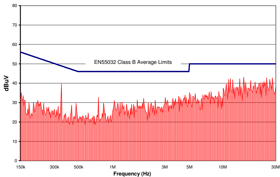
Figure 18. CPE20A18 Conducted Emissions using above specified input filter, V_{in} = 24V , Full Resistive Load
