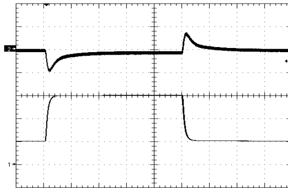
Figure 12. Load Transient Response (100mV/div), di/dt=0.1A/uS, 25% - 75% - 25% of full load, +4700uF, time scale: 200uS/div. Ch1=5A/div
