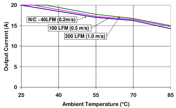
Figure 4. Output Current Derating vs Ambient Temperature & Airflow (air flowing from pin 3 to pin 1, Vin = 12 V, without baseplate)
