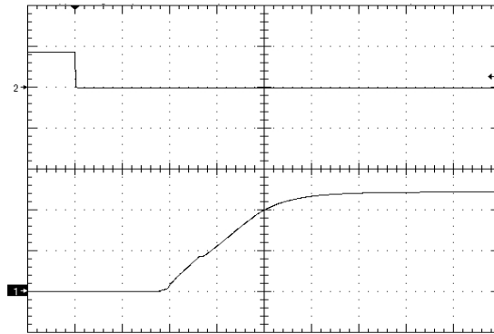
Figure 10. Startup Waveform via Enable Pin, time scale 4mS/div. Vin=Vin_nom, full load + 10000uF (neg. enable.) Ch1=2V/div,Ch2=5V/div
