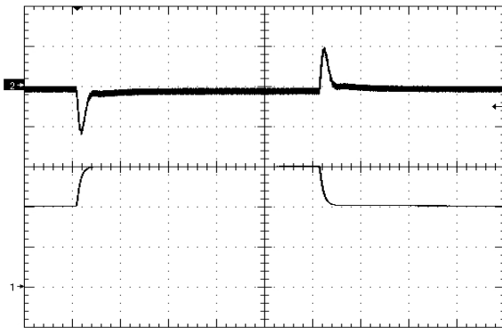
Figure 11. Load Transient Response (100mV/div), di/dt=0.1A/uS, 50% - 75% - 50% of full load, time scale: 200uS/div. Ch1=5A/div
