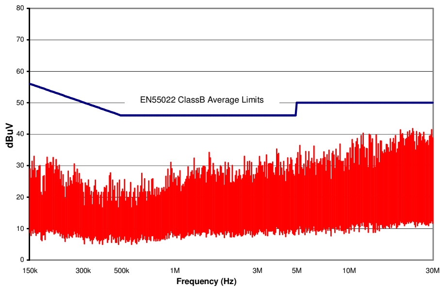
Figure 16. CPE1U48 Conducted Emissions using above specified input filter, Vin = 48V, Full Resistive Load
