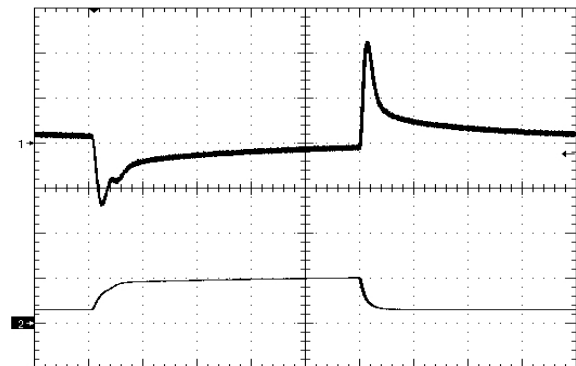
Figure 10. Load Transient Response (100mV/div), di/dt=0.1A/uS, 25% - 75% - 25% of full load, Ch2=1A/div, time scale: 200uS/div
