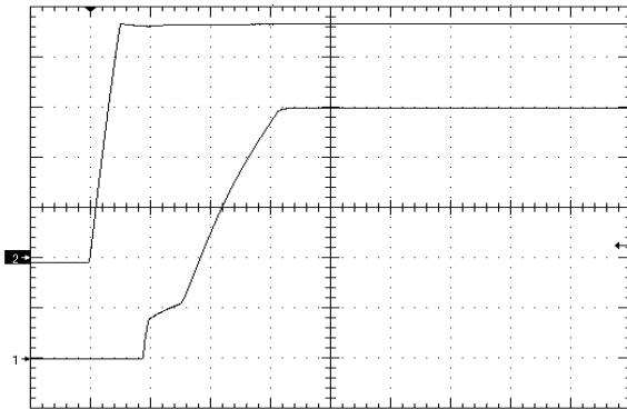
Figure 7. Startup Waveform via Line Voltage, time scale 20mS/div. Vin=Vin_nom, no load Ch1=10V/div, Ch2=10V/div
