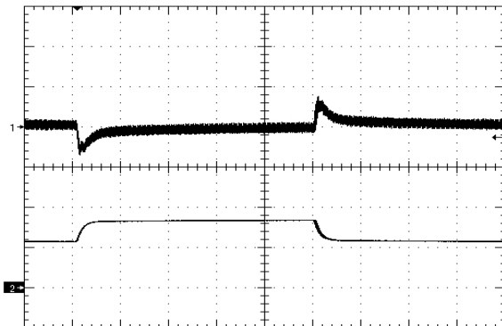
Figure 9. Load Transient Response (100mV/div), di/dt=0.1A/uS, 50% - 75% - 50% of full load, Ch2=0.5A/div, time scale: 200uS/div
