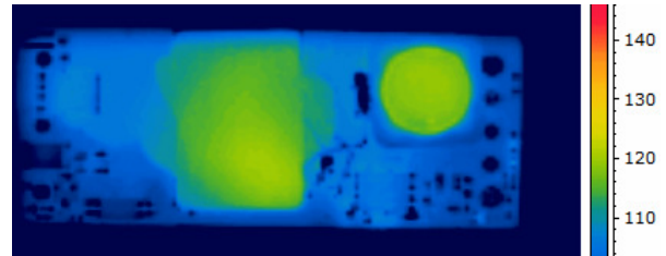
Figure 4. Thermal Image of CPE1U48 1.20A output, 70C Ambient, 200lfm airflow, Vin = 48V, airflow from pin 3 to pin 1, T max = 122°C
