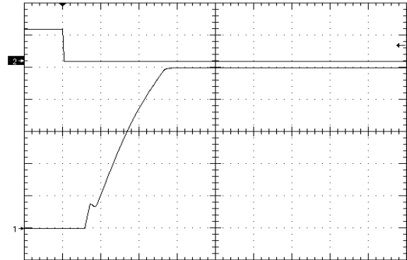
Figure 8. Startup Waveform via Enable Pin, time scale 20mS/div. Vin=Vin_nom, full res. load + 220uF, negative enbl, Ch1=10V/div, Ch2=5V/div
