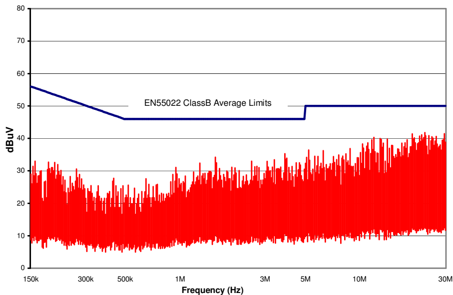
Figure 16. CPE1U48 Conducted Emissions using above specified input filter, Vin = 48V, Full Resistive Load
