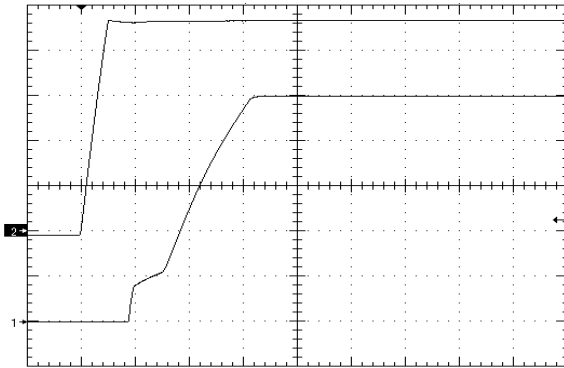
Figure 7. Startup Waveform via Line Voltage, time scale 10mS/div. Vin=Vin_nom, no load Ch1=10V/div, Ch2=10V/div
