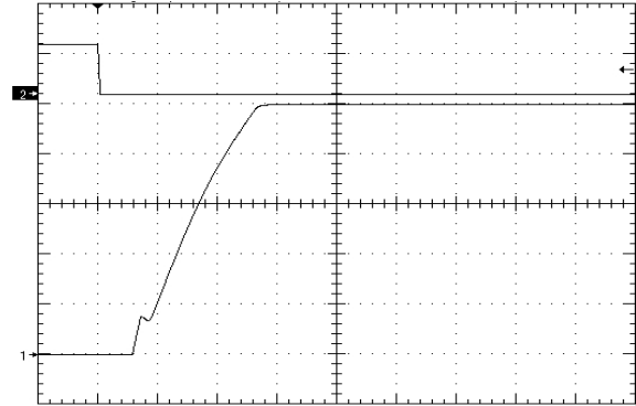
Figure 8. Startup Waveform via Enable Pin, time scale 10mS/div. Vin=Vin_nom, full res. load + 220uF, negative enbl, Ch1=10V/div, Ch2=5V/div
