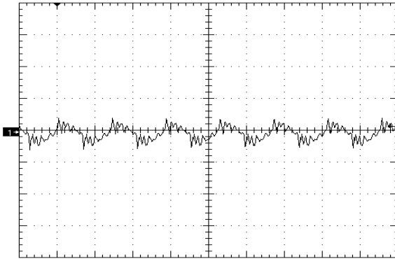
Figure 5. Output Voltage Ripple (200mV/div), time scale – 2uS/div. Vin=Vin_nom, full resistive.
