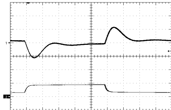
Figure 10. Load Transient Response (100mV/div), di/dt=0.1A/uS, 25% - 75% - 25% of full load +220uF Ch2=1A/div, time scale: 200uS/div
