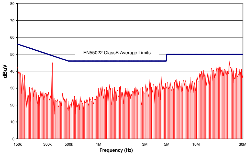
Figure 16. CPE1U24 Conducted Emissions using above specified input filter, Vin = 24V, Full Resistive Load
