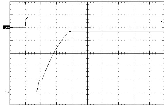
Figure 8. Startup Waveform via Enable Pin, time scale 10mS/div. Vin=Vin_nom, full res. load + 220uF, positive enbl, Ch1=10V/div, Ch2=5V/div
