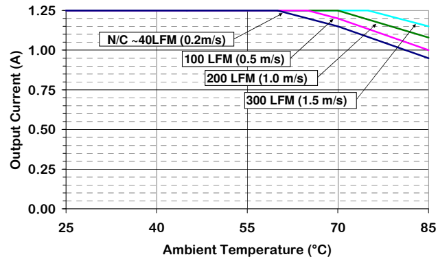
Figure 3. Output Current Derating vs Ambient Temperature & Airflow (converter mounted vertically with air flowing from pin 3 to pin 1, Vin = 24 V.)
