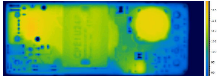
Figure 4. Thermal Image of CPE1U24 1.25A output, 70C Ambient, 200lfm airflow, Vin = 24V, airflow from pin 3 to pin 1, T max = 122°C
