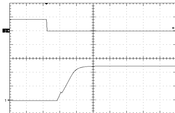
Figure 8. Startup Waveform via Line Voltage, time scale 10mS/div. Vin=Vin_nom, full resistive load + 10000uF. Ch1=2V/div,Ch2=5V/div
