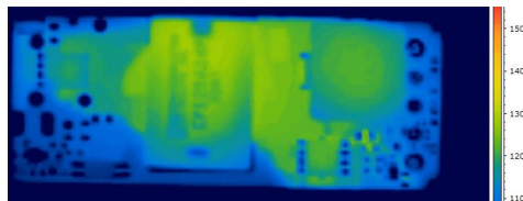
Thermal Image of module @ 48Vin, 100LFM & 85C
