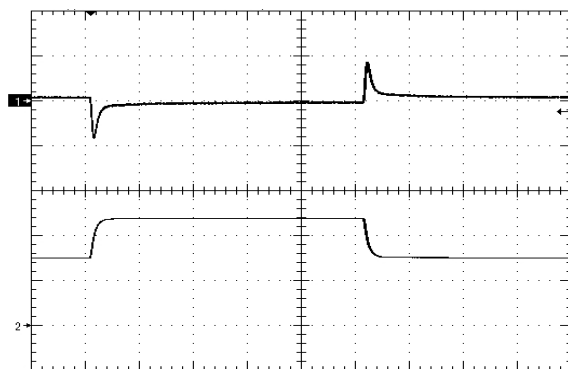
Figure 10. Load Transient Response di/dt=0.1A/uS, 50% - 75% - 50% of full load, time scale: 200uS/div Ch1=100mV/div, Ch2=5A/div
