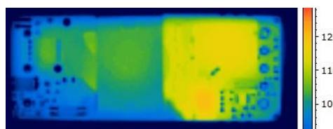
Thermal Image of module @ 48Vin, 200LFM & 70C
