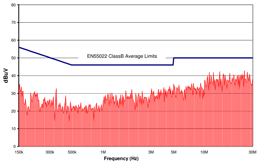
Figure 18. CPE15A36 Conducted Emissions using above specified input filter, Vin = 48V, Full Resistive Load
