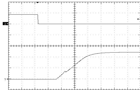
Figure 10. Startup Waveform via Enable Pin, time scale 4mS/div. Vin=Vin_nom, full load + 10000uF (neg. enable.) Ch1=2V/div,Ch2=5V/div
