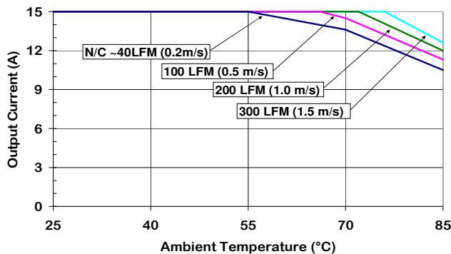
Figure 5. Output Current Derating vs Ambient Temperature & Airflow (air flowing from pin 3 to with pin 1, Vin = 24 V, with baseplate)
