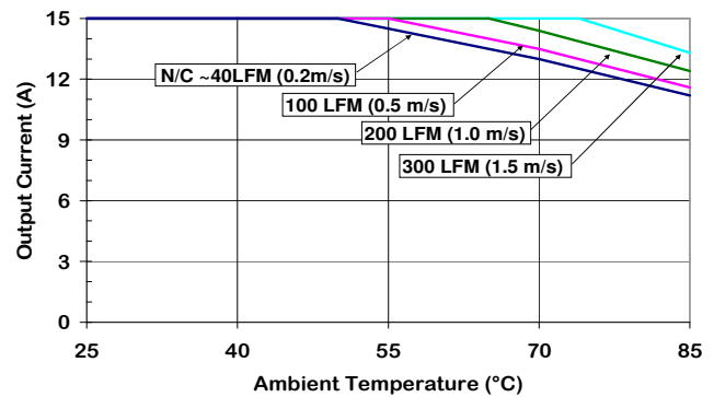
Figure 4. Output Current Derating vs Ambient Temperature & Airflow (air flowing from pin 3 to pin 1, Vin = 12 V, without baseplate)
