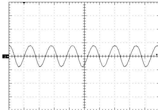
Figure 8. Input Reflected Ripple Current (20mA/div) time scale - 2uS/div. Vin=Vin_nom, full resistive.
