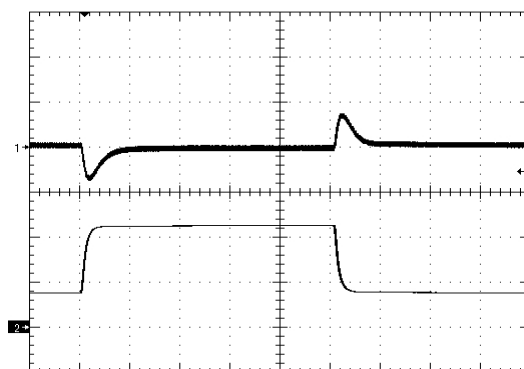
Figure 12. Load Transient Response (100mV/div), di/dt=0.1A/uS, 25% - 75% - 25% of full load, +4700uF, time scale: 200uS/div
