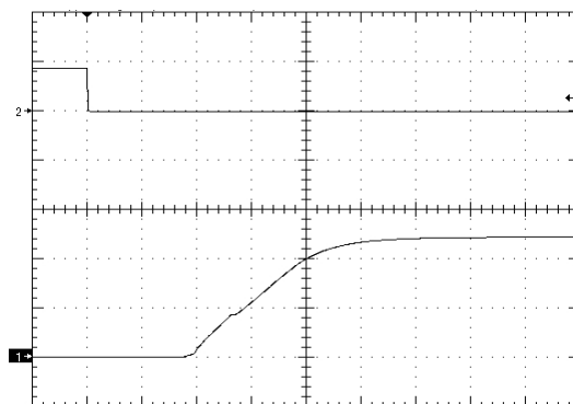
Figure 10. Startup Waveform via Enable Pin, time scale 4mS/div. Vin=Vin_nom, full load + 10000uF (neg. enable.) Ch1=2V/div,Ch2=5V/div
