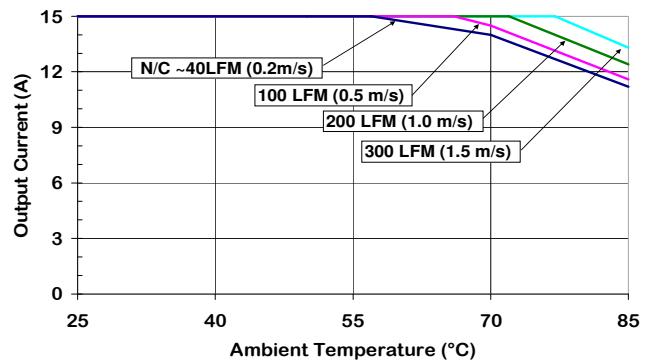
Figure 6. Output Current Derating vs Ambient Temperature & Airflow (air flowing from pin 3 to with pin 1, Vin = 12 V, with baseplate)
