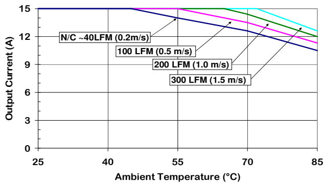
Figure 3. Output Current Derating vs Ambient Temperature & Airflow (air flowing from pin 3 to pin 1, Vin = 24 V, without baseplate)
