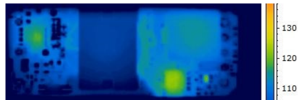
Thermal Image of module @ 24Vin, 100LFM & 55C
