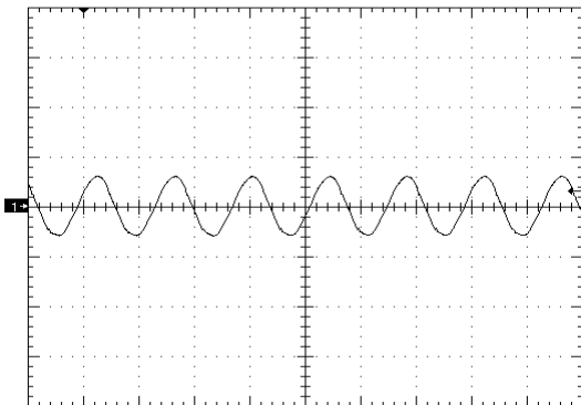
Figure 7. Output Voltage Ripple (50mV/div), time scale – 2uS/div. Vin=Vin_nom, full resistive.
