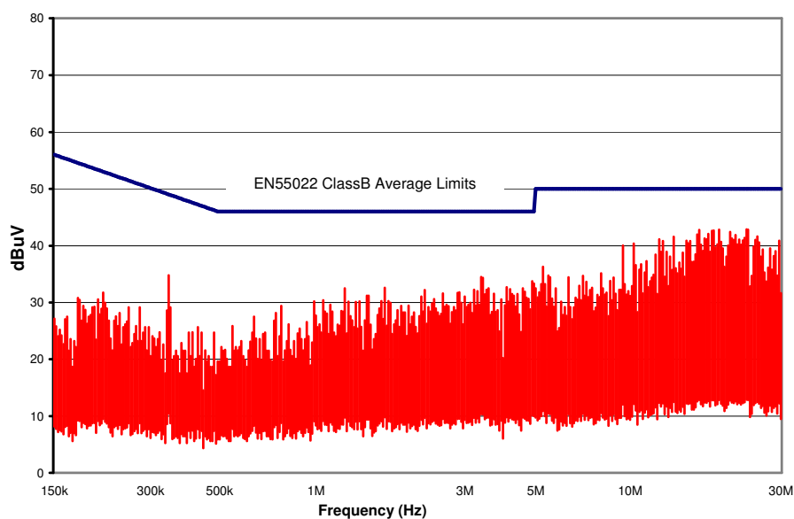
Figure 18. CPE15A18 Conducted Emissions using above specified input filter, Vin = 24V, Full Resistive Load
