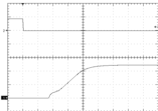
Figure 9. Startup Waveform via Enable Pin, time scale 4mS/div. Vin=Vin_nom, full resistive load (negative enable.) Ch1=2V/div,Ch2=5V/div
