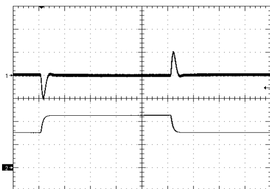
Figure 11. Load Transient Response (100mV/div), di/dt=0.1A/uS, 50% - 75% - 50% of full load, time scale: 200uS/div.
