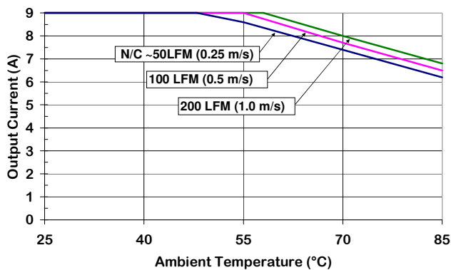
Figure 4. Output Current Derating vs Ambient Temperature & Airflow (Open Frame module) Vin = 12 V
