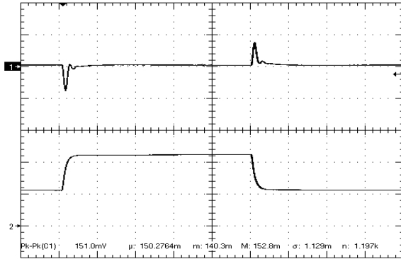
Figure 13. Load Transient Response (100mV/div), di/dt=0.1A/uS, 25%-50%-25% of full load, Cout=Fig16 time scale: 200uS/div. Ch1=Vout, Ch2=Iout (2A/div)
