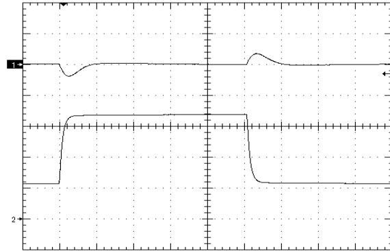
Figure 14. Load Transient Response 100mV/div), di/dt=0.2A/uS, 25% - 75% - 25% of full load +2000uF low ESR Oscon, time scale: 200uS/div. Ch1=Vout, Ch2=Iout (2A/div)
