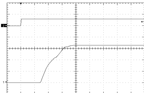
Figure 9. Startup Waveform via Enable Pin, time scale 2mS/div. Vin=Vin_nom, Iout=no load Cout=0, Ch1=Vout (1V/div), Ch2=enable (10V/div)
