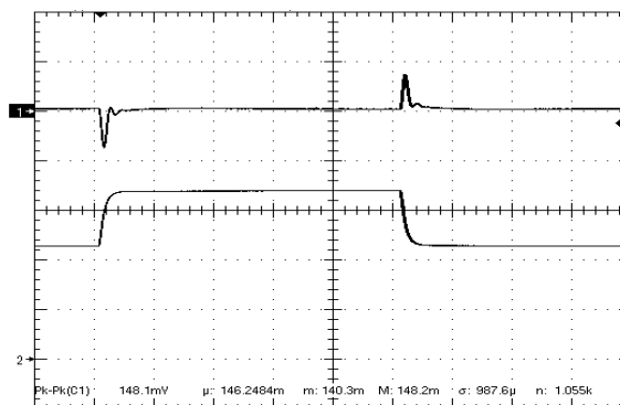
Figure 12. Load Transient Response (100mV/div), di/dt=0.1A/uS, 50%-75%-50% of full load, Cout=Fig16 time scale: 200uS/div. Ch1=Vout, Ch2=Iout (2A/div)
