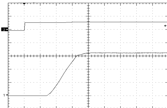
Figure 11. Startup Waveform via Enable Pin, time scale 2mS/div. Vin=Vin_nom, Iout=no load Cout=4700uF, Ch1=Vout (1V/div), Ch2=enable (10V/div)
