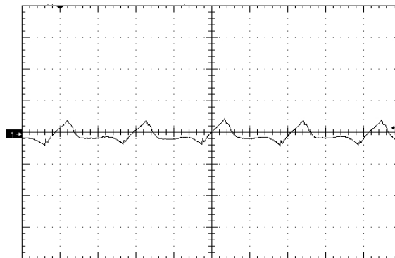
Figure 8. Output Voltage Ripple (20mV/div), time scale – 1uS/div. Vin=Vin_nom, full load Cout=1uF ceramic + 10uF Tantalum (see Fig 16)
