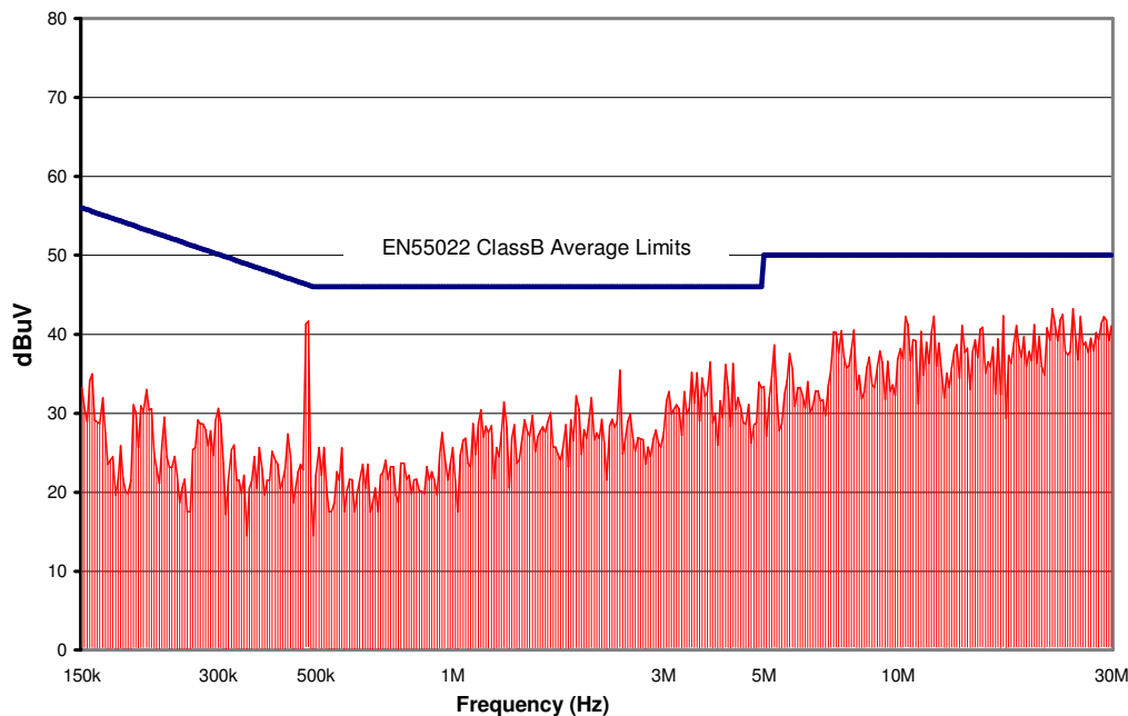
Figure 20. CP40_1790018 Conducted Emissions using above specified input filter. Vin = 24V, Full Resistive Load
