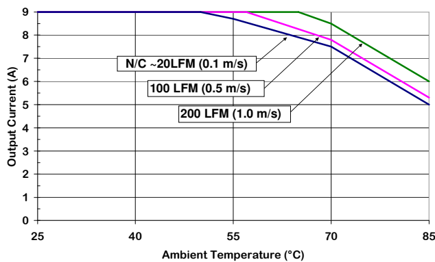
Figure 5. Output Current Derating vs Ambient Temperature & Airflow (Encapsulated module) Vin = 12V, 24V
