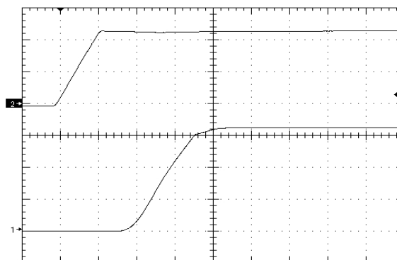
Figure 10. Startup Waveform via Input Voltage, time scale 2mS/div. Vin=Vin_nom, Iout=full load Cout=4700uF, Ch1=Vout (1V/div), Ch2=Vin (10V/div)
