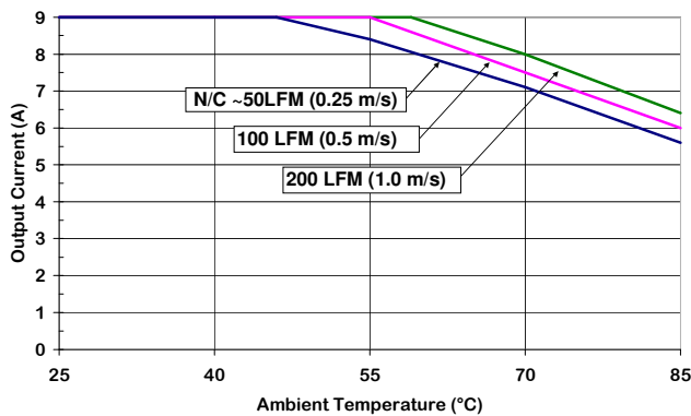
Figure 3. Output Current Derating vs Ambient Temperature & Airflow (Open Frame module) Vin = 24 V
