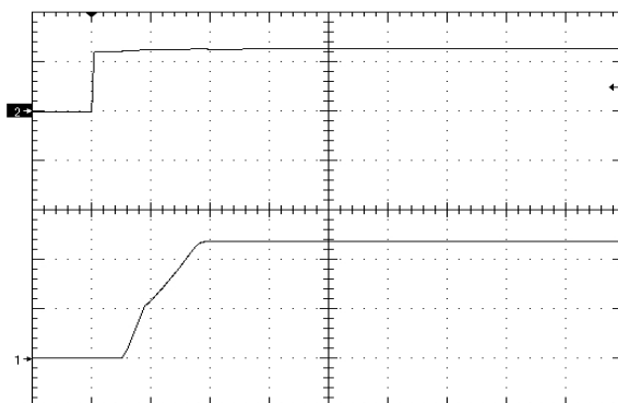
Figure 11. Startup Waveform via Enable Pin, time scale 4mS/div. Vin=Vin_nom, Iout=full load Cout=2200uF, Ch1=Vout (5V/div), Ch2=Enable (5V/div)
