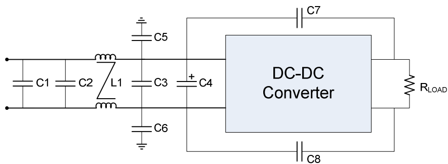
Figure 19. EMI Filter
