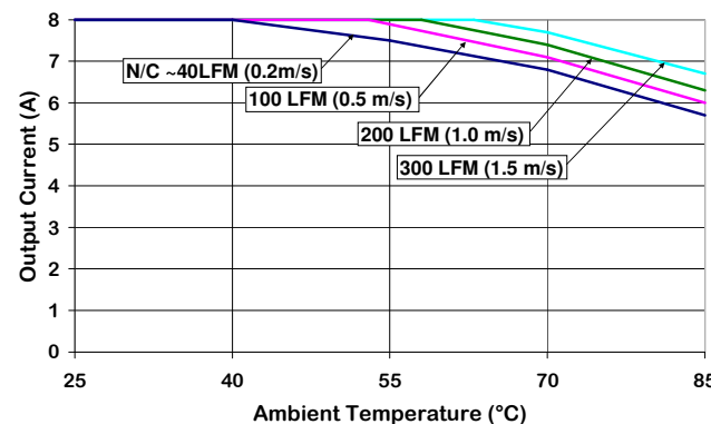
Figure 4. Output Current Derating vs Ambient Temperature & Airflow (Open Frame module) Vin = 12 V (airflow from pin 1 to pin 2)
