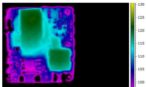
Figure 6. Thermal Image of CP30B1225036 2.5A output, 70C Ambient, 200lfm airflow, Vin = 48V, T max = 122°C
