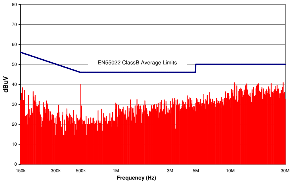
Figure 20. CP30_1225036 Conducted Emissions using above specified input filter. Vin = 48V, Full Resistive Load
