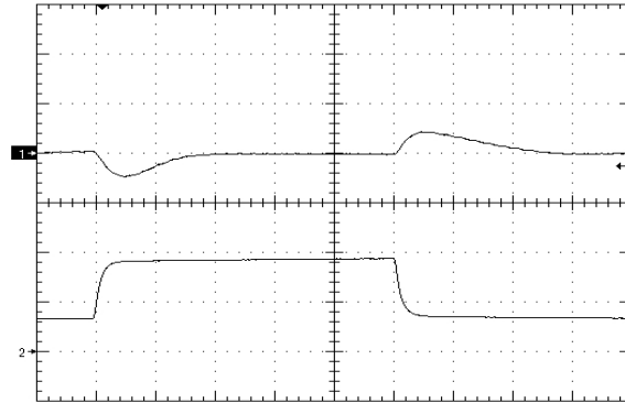
Figure 14. Load Transient Response 100mV/div), di/dt=0.2A/uS, 25% - 75% - 25% of full load +1000uF low ESR Oscon, time scale: 200uS/div. Ch1=Vout, Ch2=Iout (1A/div)
