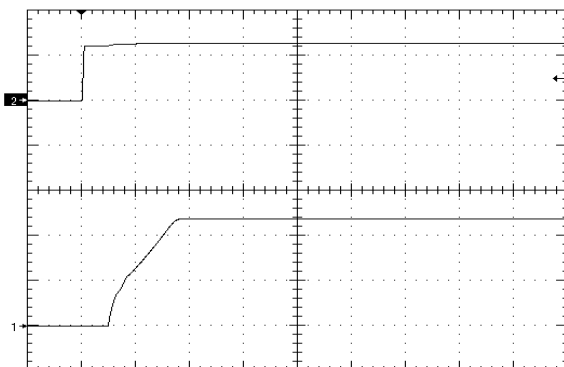
Figure 9. Startup Waveform via Enable Pin, time scale 4mS/div. Vin=Vin_nom, Iout=no load Cout=0, Ch1=Vout (5V/div), Ch2=Enable (5V/div)
