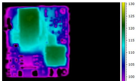
Figure 6. Thermal Image of CP15B1213036 1.3A output, 85C Ambient, 100lfm airflow, Vin = 48V, T_{max} = 118^{\circ}C
